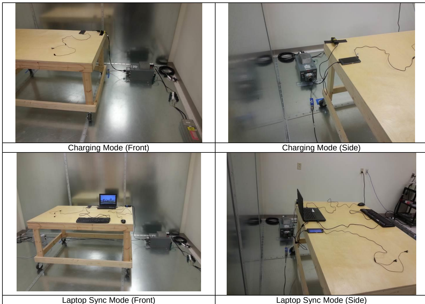
Figure 1 Test Setup for Conducted Emissions
