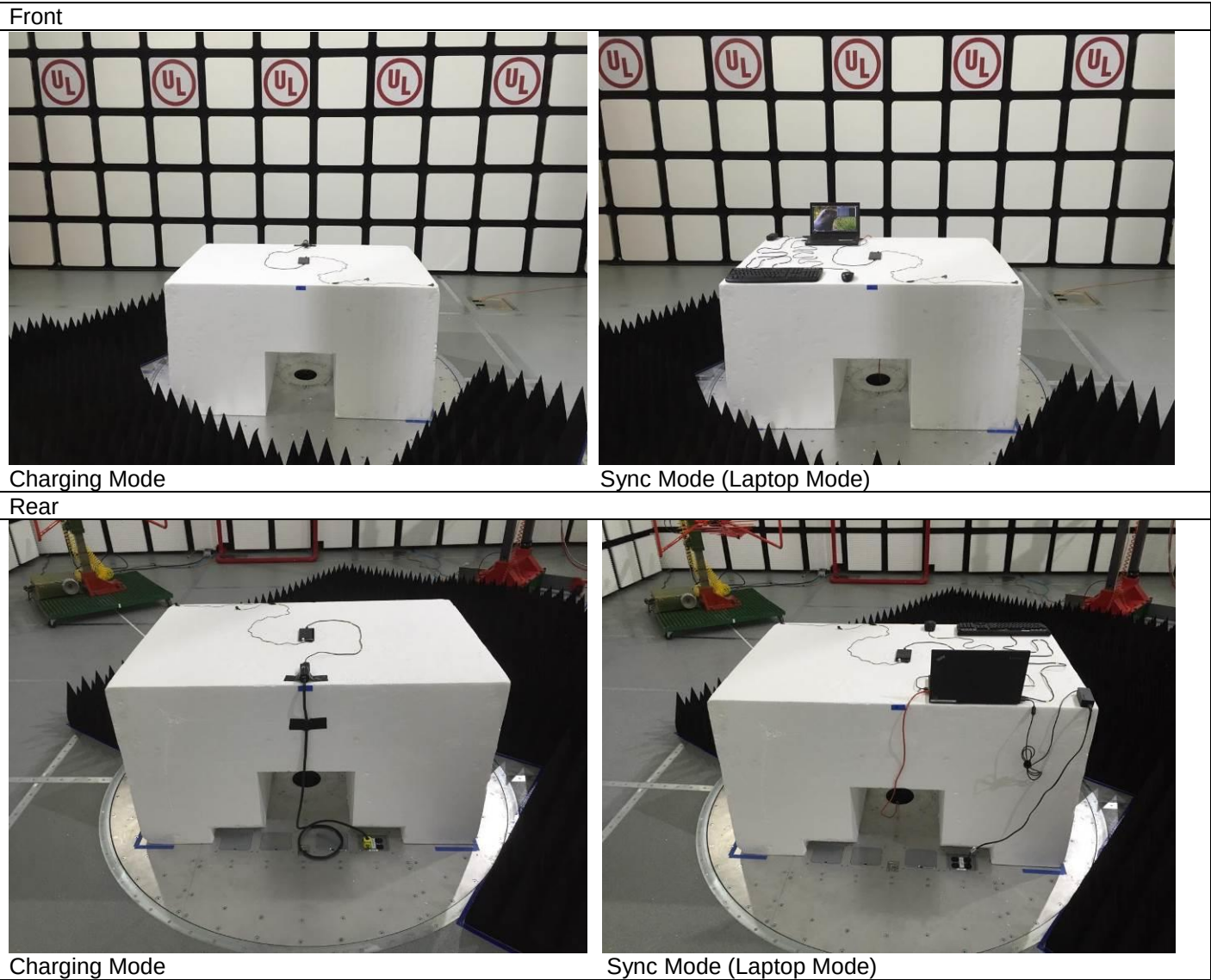
Figure 5 Test setup for Radiated Emissions > 1GHz
