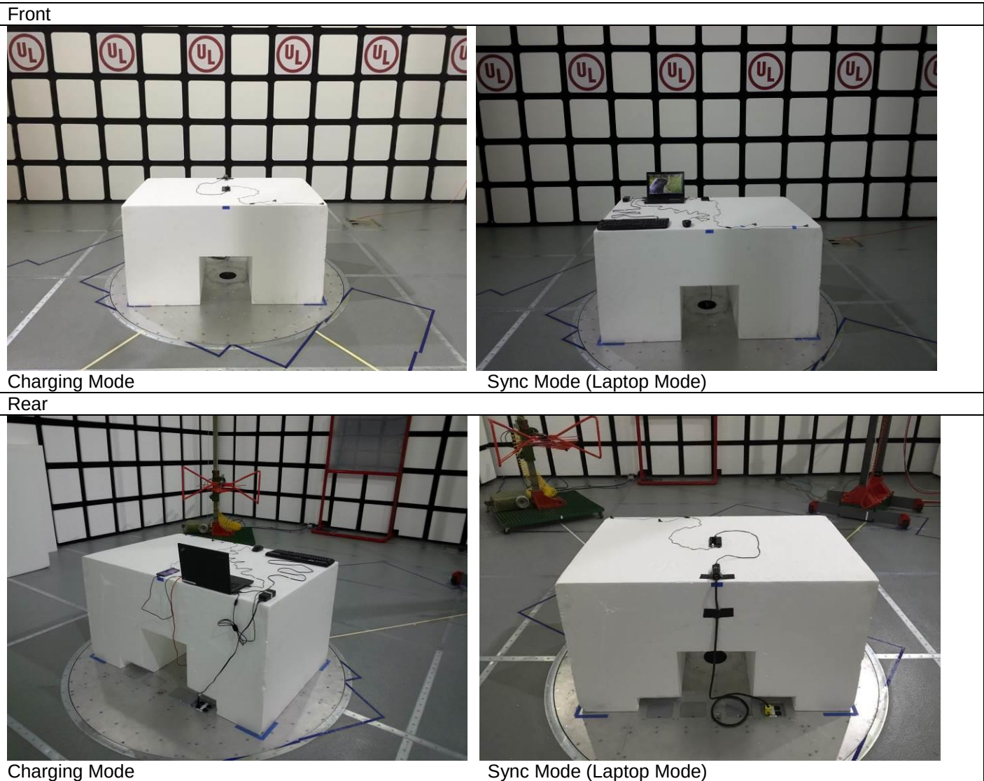
Figure 4 Test setup for Radiated Emissions < 1GHz
