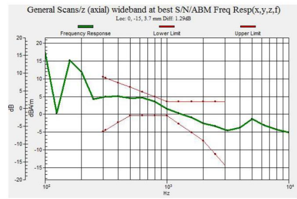
Fig 7.4 WCDMA Band V Ch4182
