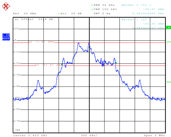
20 dB Bandwidth Plot on 2403MHz
