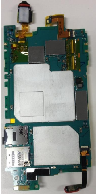
Internal PWB with Shield cases (Front-side)
