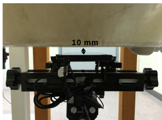
Fig.11 EUT back with headset to flat phantom
