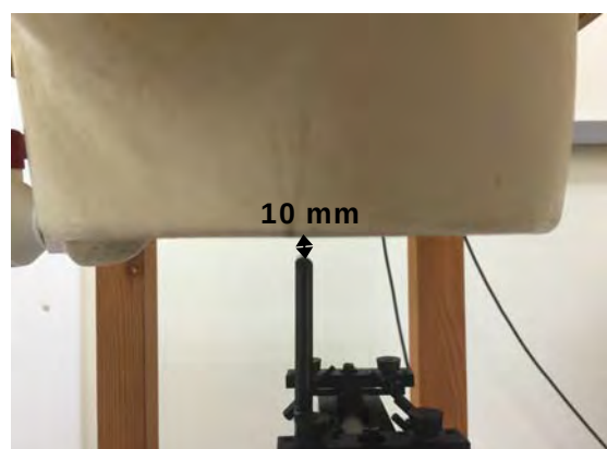
Fig.14 EUT bottom to flat phantom
