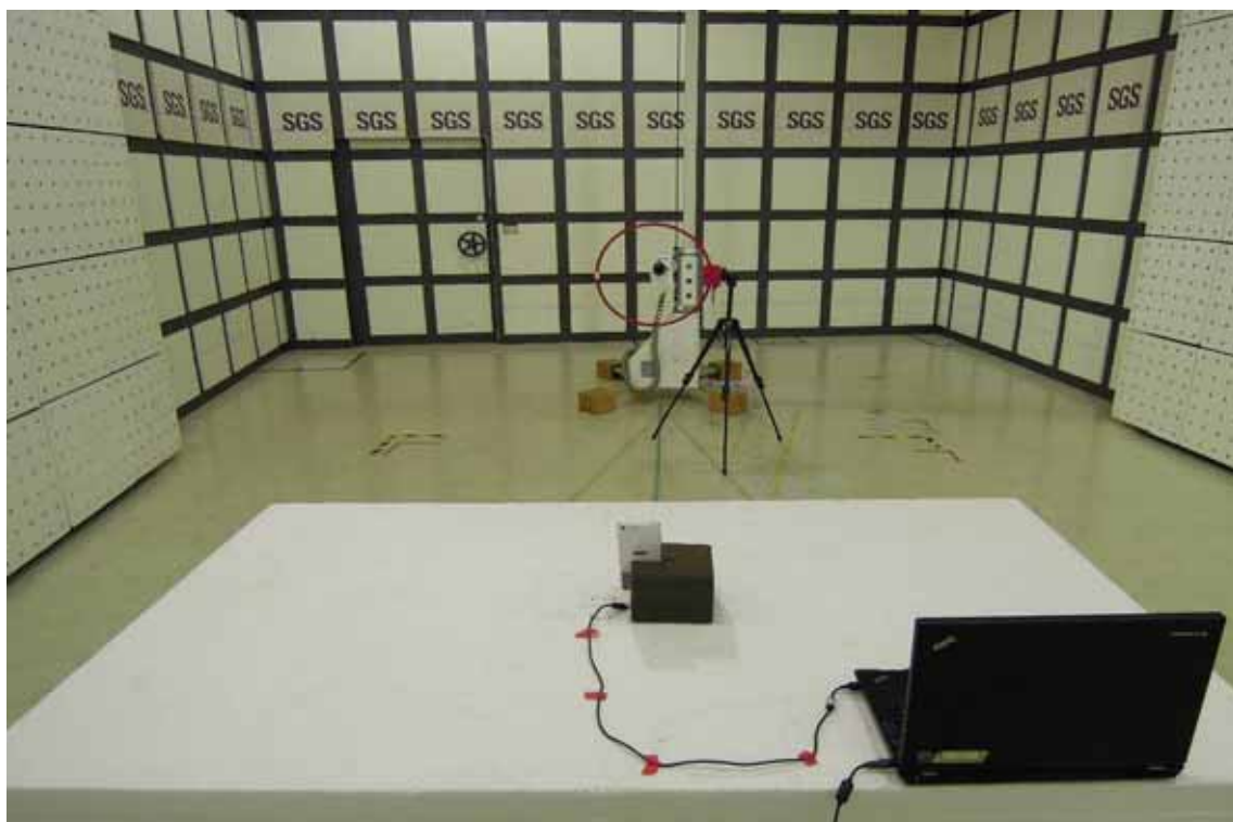
Antenna with H polarization
