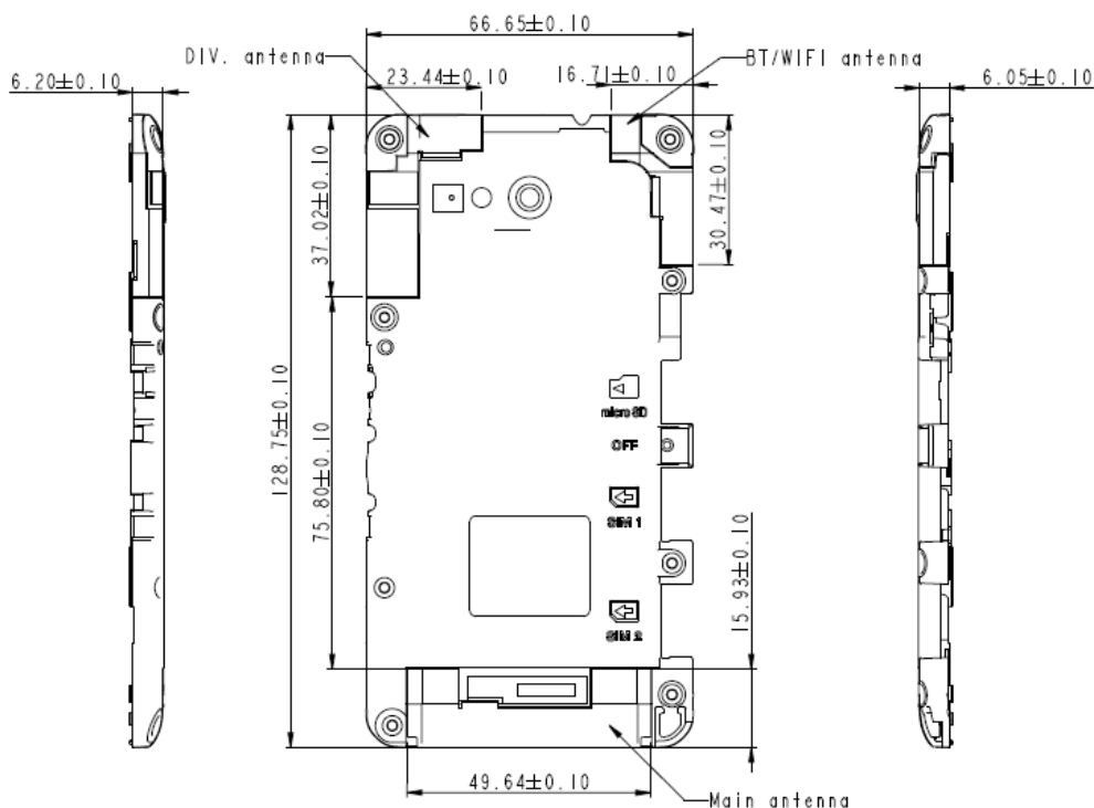
Fig.19 Antenna position of EUT (Front-Side)
