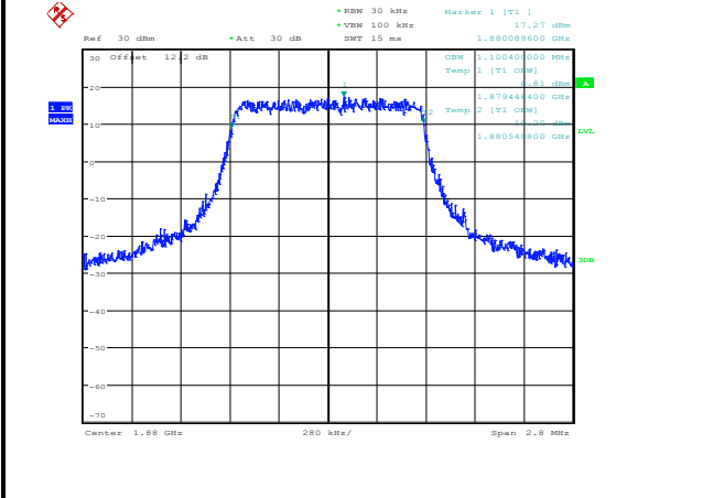
Highest Channel / 1.4MHz / QPSK
