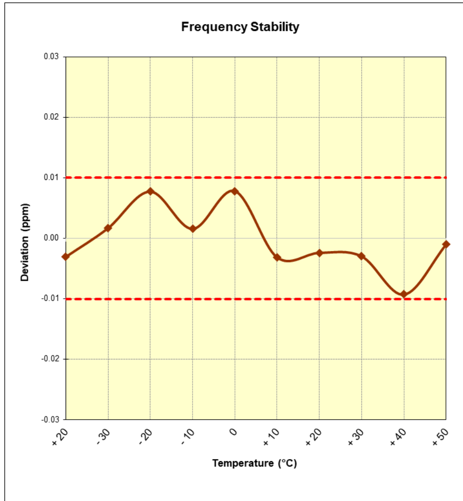
Figure 7-3. Frequency Stability Plot
