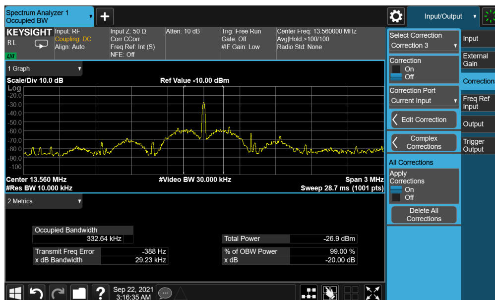
Figure 7-2. Occupied Bandwidth Plot
