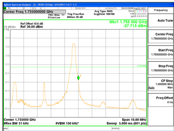
LTE B4 5MHz QPSK High Channel 1RB
