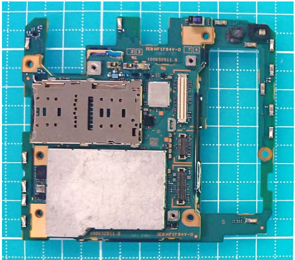
Internal Main-PWB with Shield cases (Front-side)
