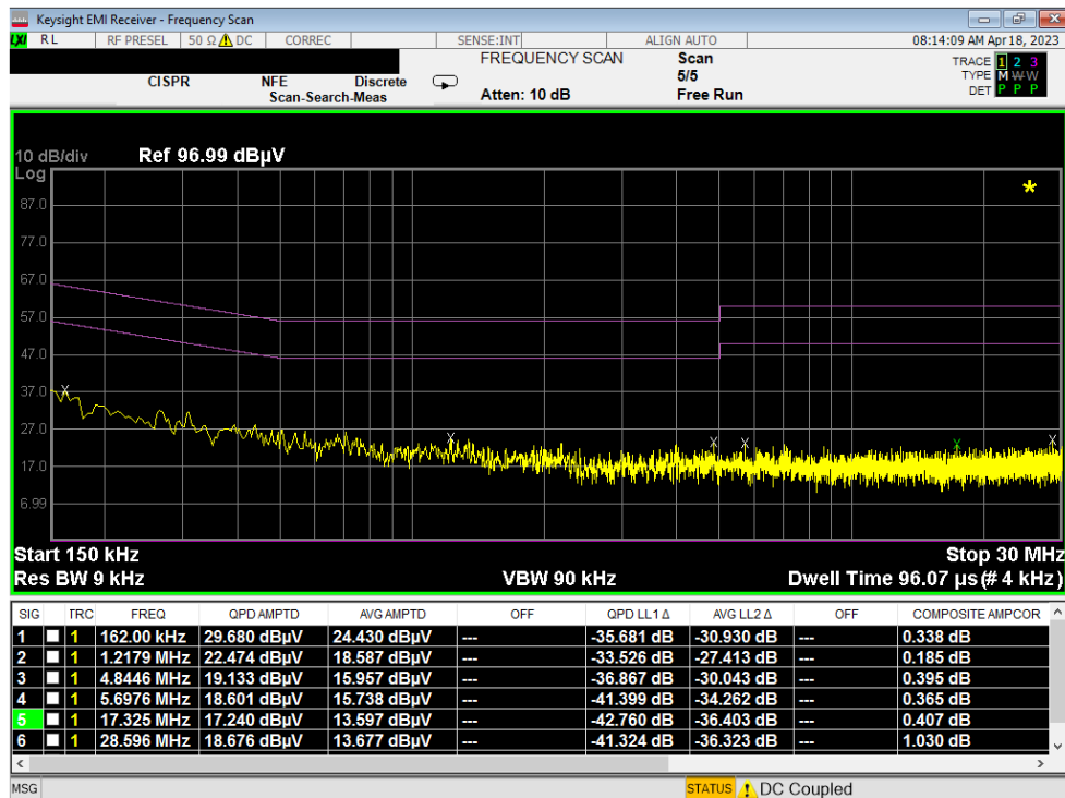
Plot 7-6. Line Conducted Plot (N) _Case #2
