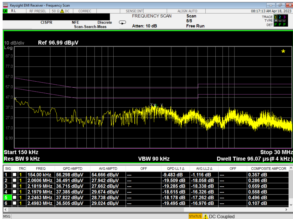
Plot 7-4. Line Conducted Plot (N) _Case #1
