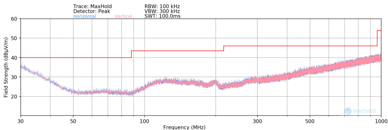
Plot 7-1. Radiated Spurious Plot Below 1GHz Case #1
