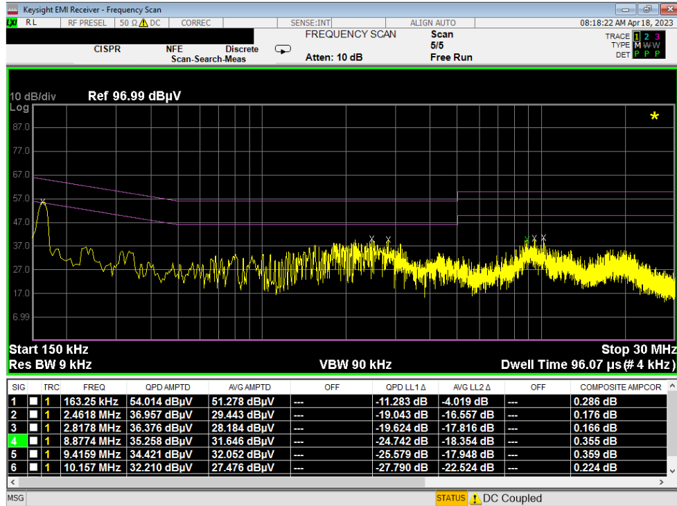
Plot 7-3. Line Conducted Plot (L1) _Case #1
