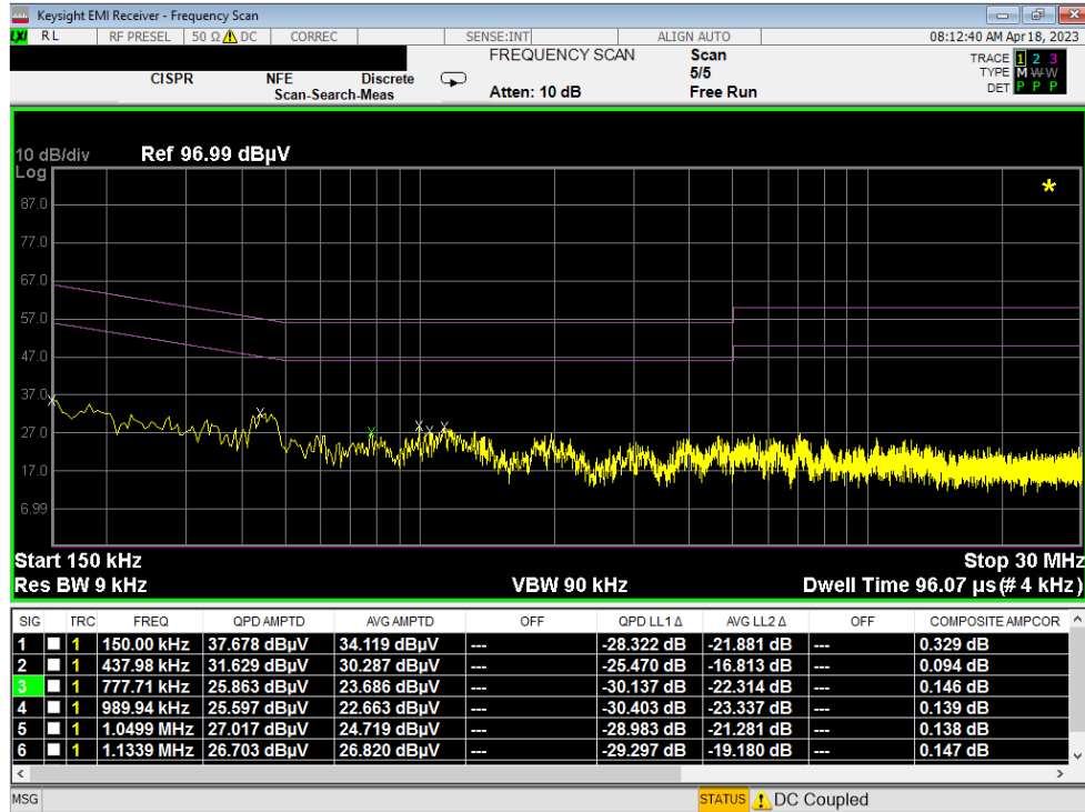
Plot 7-5. Line Conducted Plot (L1) _Case #2
