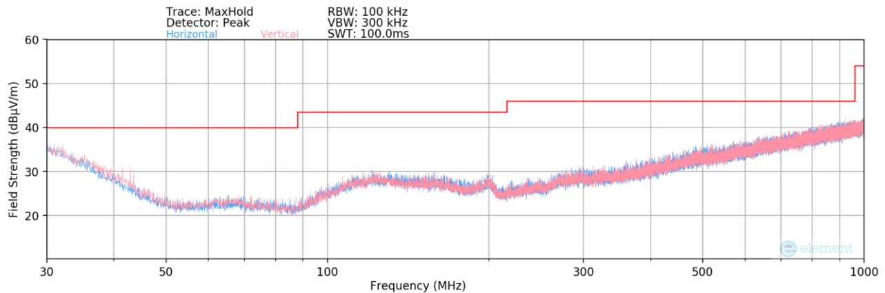
Plot 7-2. Radiated Spurious Plot Below 1GHz Case #2
