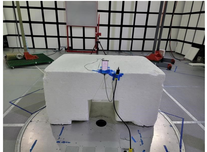
BL30 Setup 90 Degrees
