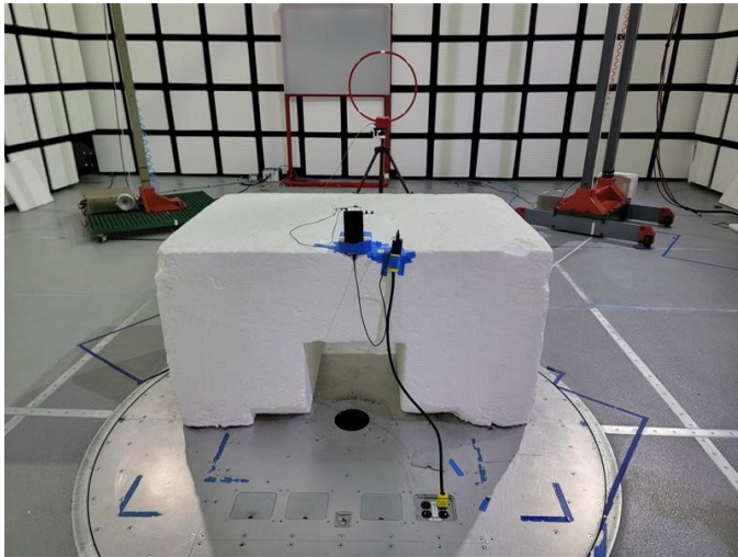
BL30 Setup 0 Degrees
