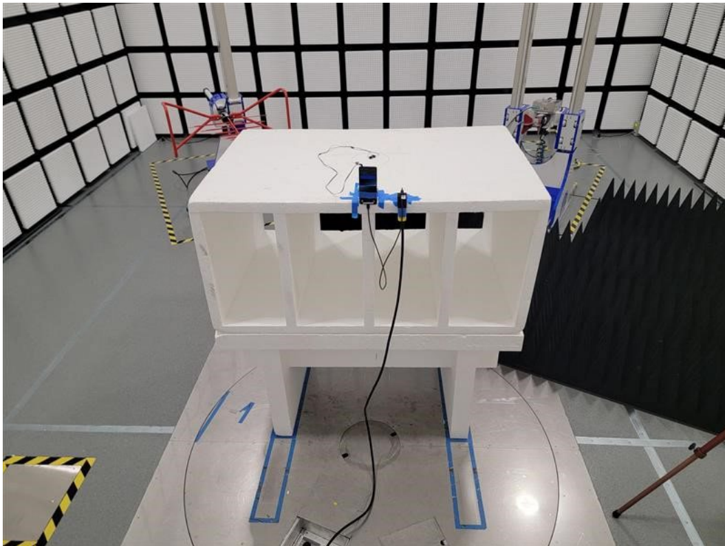
A1G Setup Front Low Band
