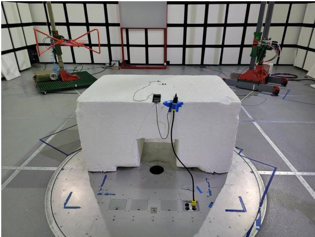
BL1G Setup Back (Mid Band)
