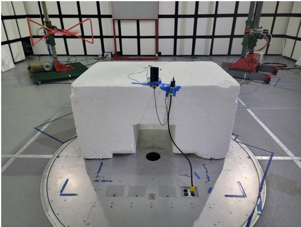
BL1G Setup Back (Low Band)
