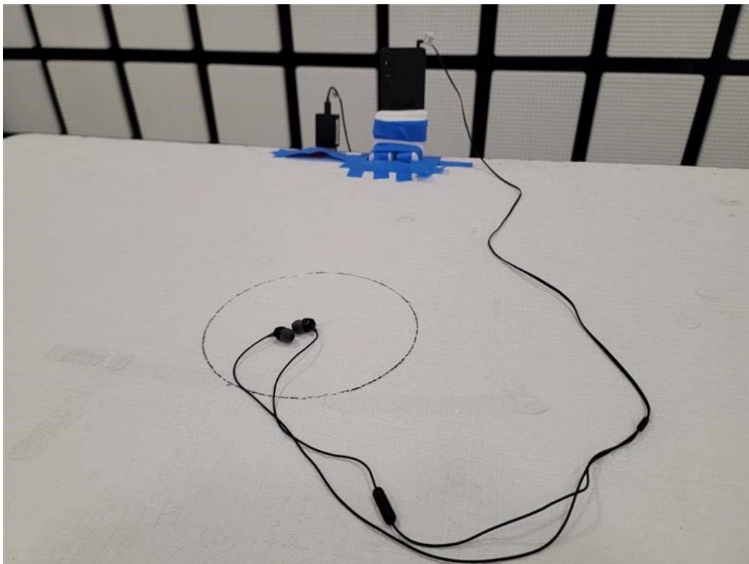
A1G Setup Back Low Band
