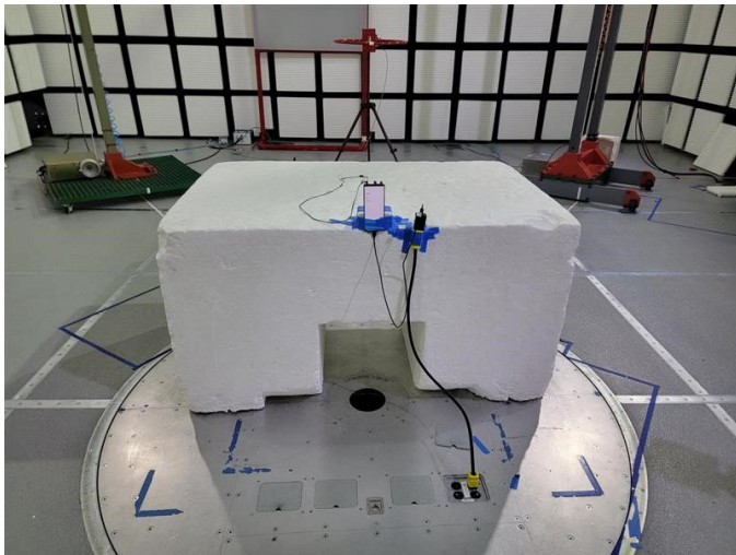
BL30 Setup Flat
