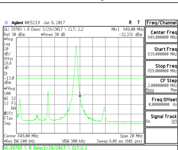
LTE B26 10MHz 16QAM High Channel 1RB
