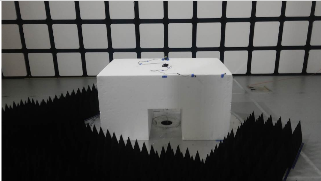
Figure 9 Test setup for Radiated Emissions > 1GHz Charger
