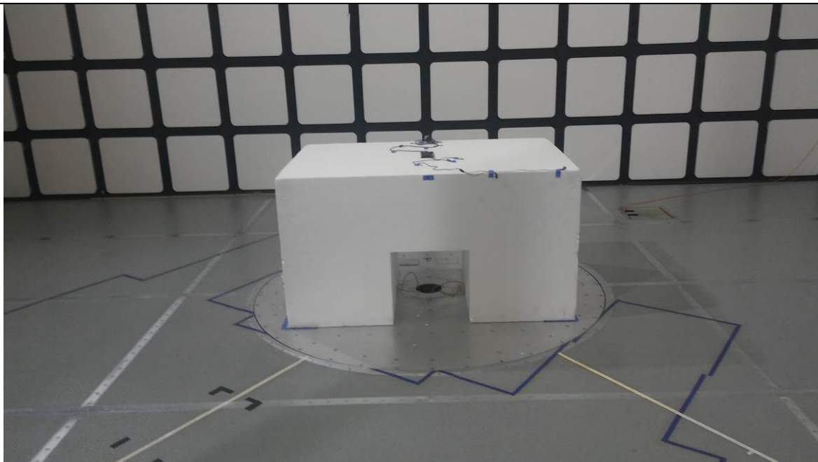
Figure 7 Test setup for Radiated Emissions < 1GHz Charger
