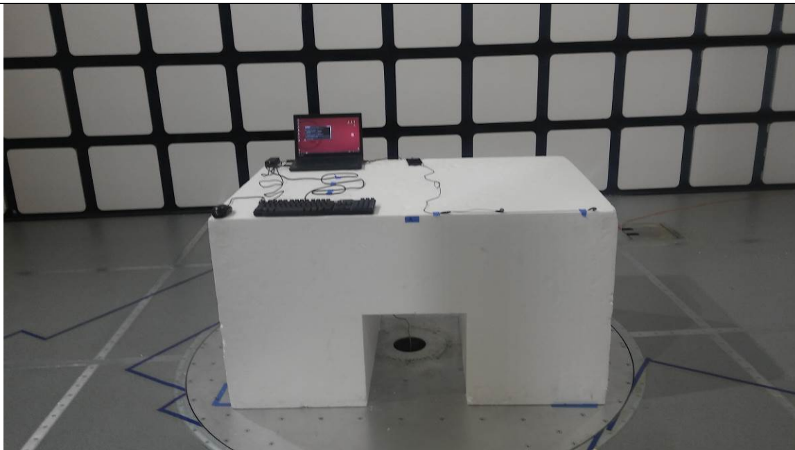
Figure 8 Test setup for Radiated Emissions < 1GHz Sync
