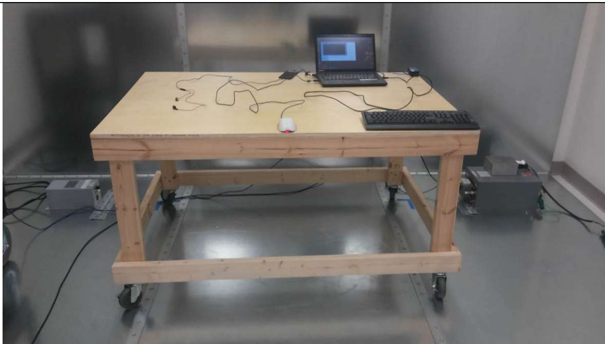
Figure 2 Test Setup for Conducted Emissions -Sync
