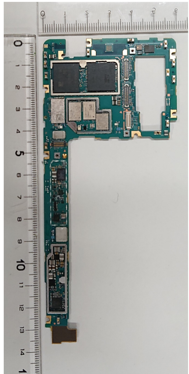
Internal PWB without Shield cases (Front-side)
