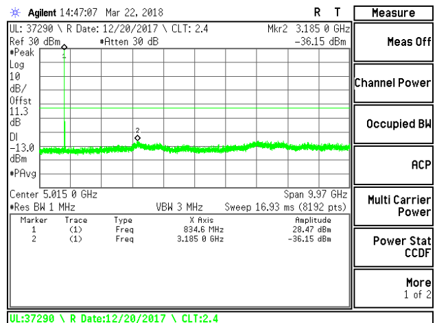
LTE B5 5MHz 16QAM Middle Channel RB1-0
