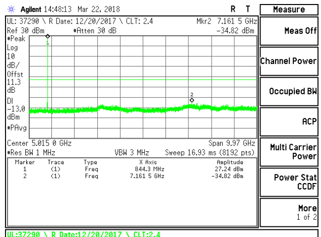
LTE B5 5MHz 16QAM High Channel RB1-0
