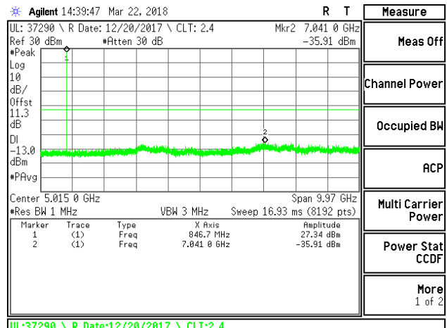
LTE B5 3MHz 16QAM High Channel RB1-0
