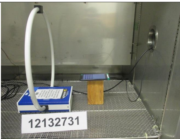
FREQUENCY TOLERANCE OVER EXTREME CONDITIONS
