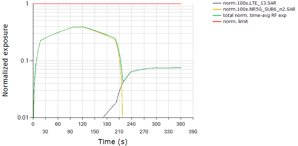
Total Normalized Time-averaged RF Exposure Tech: LTE, Band 13 / Tech: NR5G SUB6, Band n2
