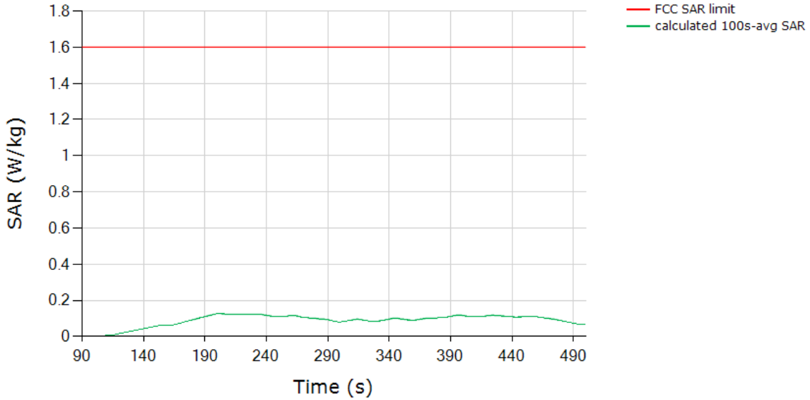
SAR (Test Sequence 2) Tech: LTE, Band 13
