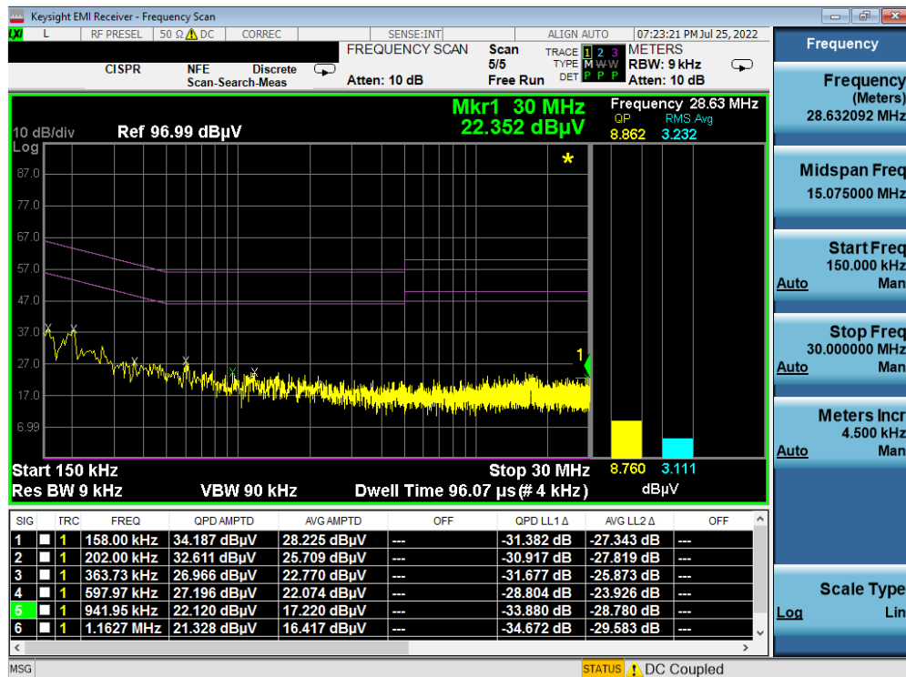
Plot 7-4. Line Conducted Plot (N)_ Case #2
