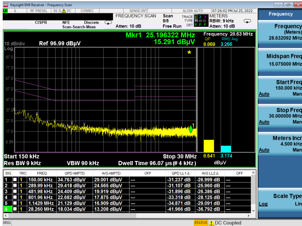
Plot 7-3. Line Conducted Plot (L1) _ Case #2
