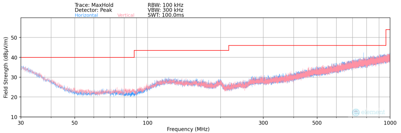
Plot 7-2. Radiated Spurious Plot Below 1GHz Case #2
