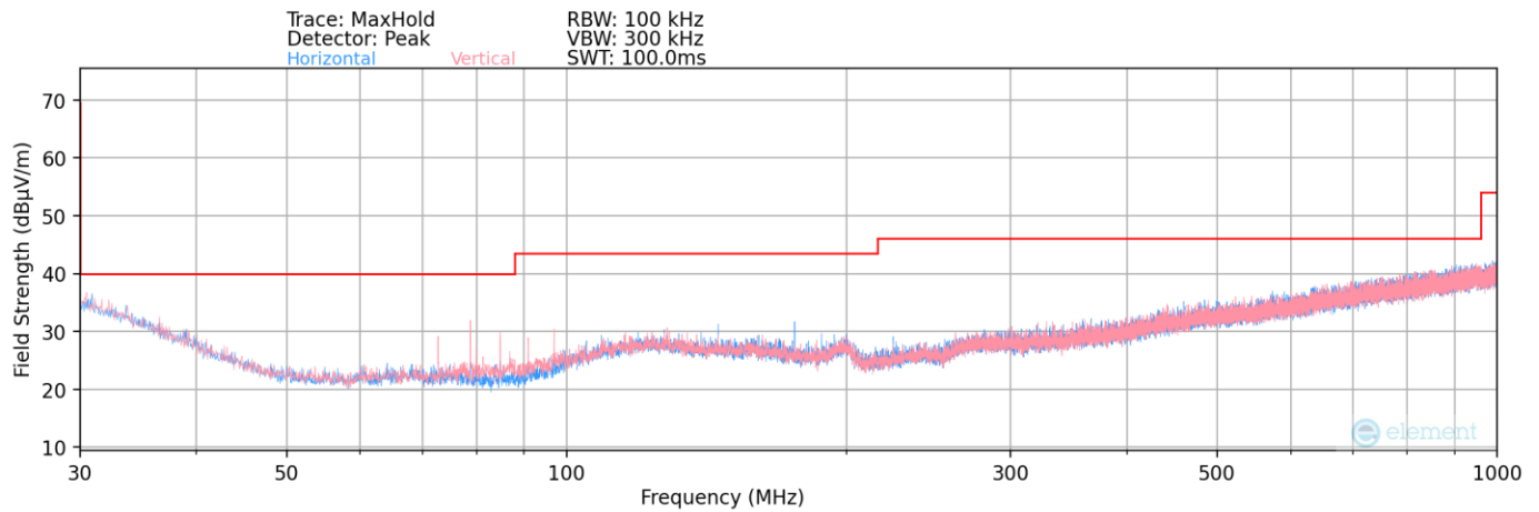
Plot 7-1. Radiated Spurious Plot Below 1GHz Case #1
