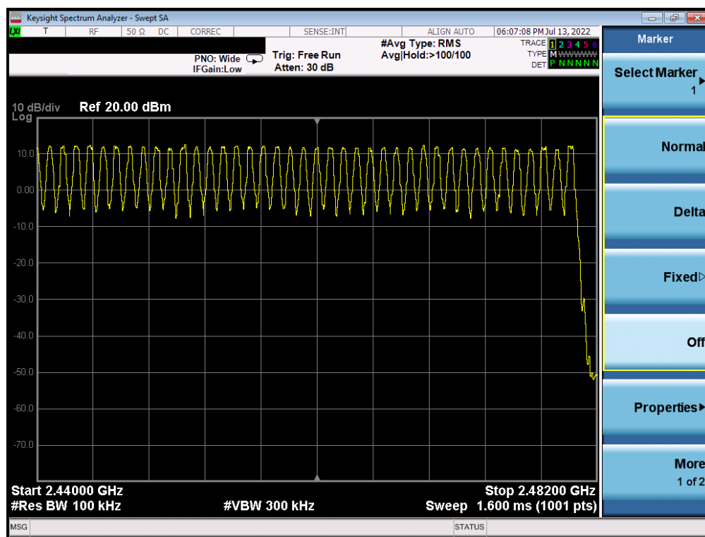
Plot 7-70. High End Spectrum Channel Hopping Plot (Bluetooth) – ANT 2
