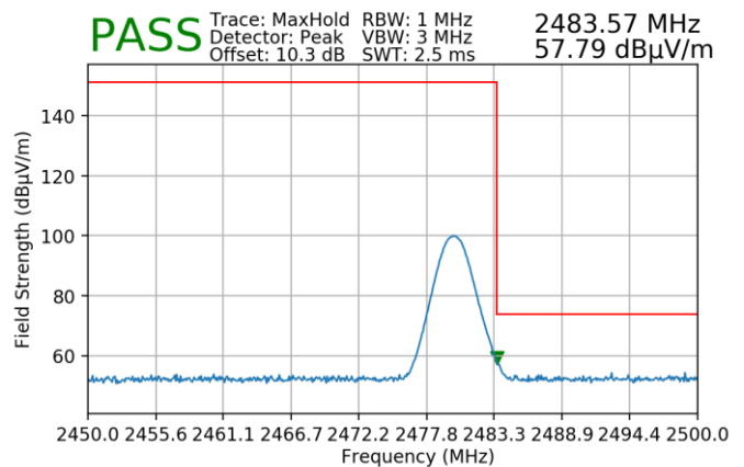
Plot 7-94. Radiated Restricted Upper Band Edge Measurement (Peak) with WCP – ANT 1
