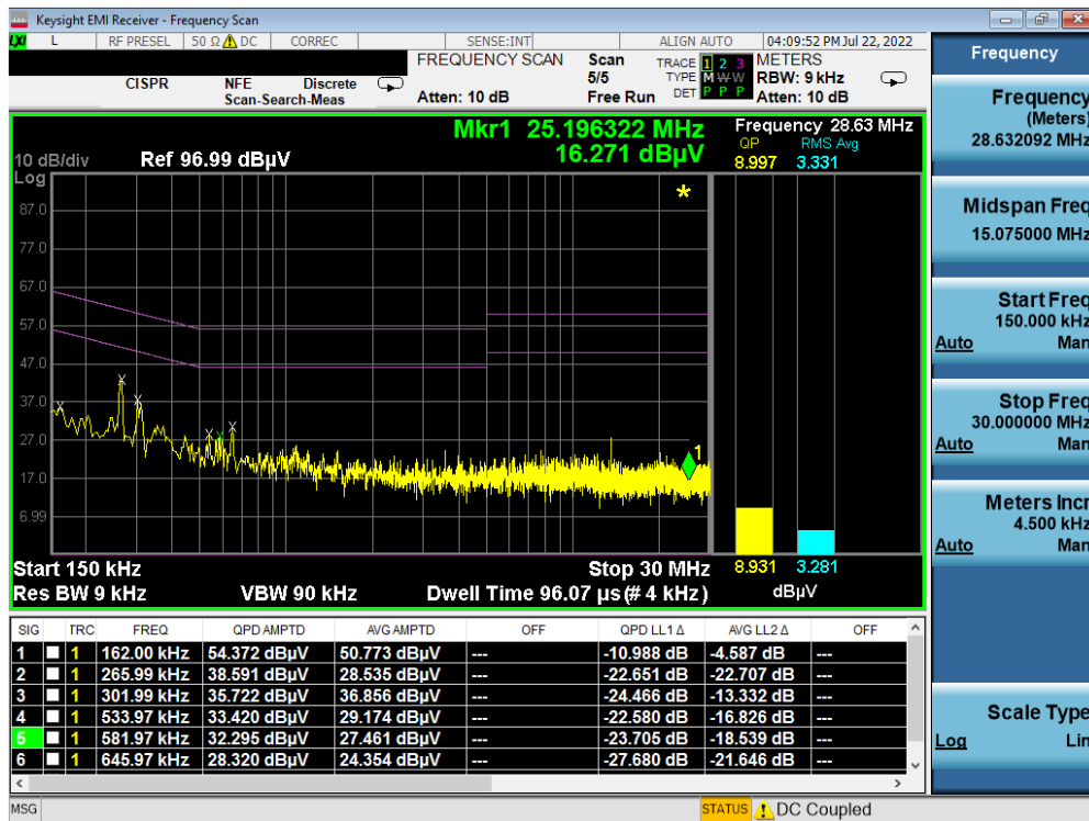
Plot 7-102. Line-Conducted Test Plot (N)
