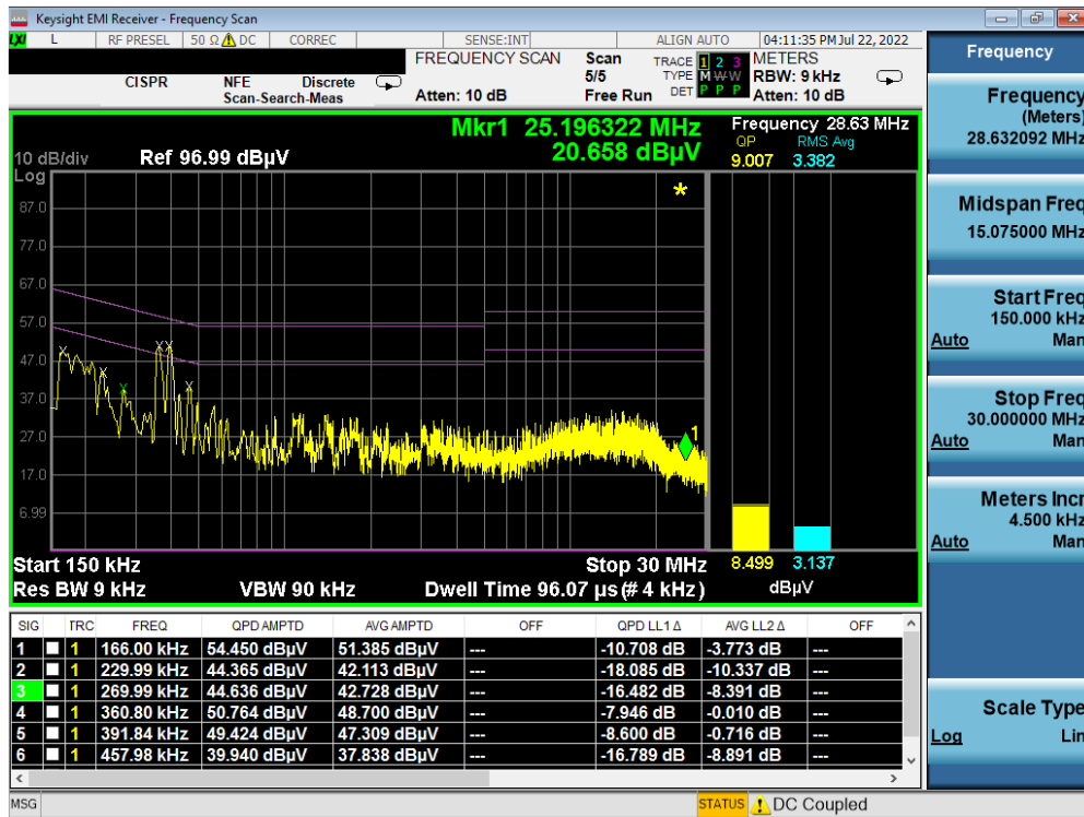
Plot 7-101. Line-Conducted Test Plot (L1)
