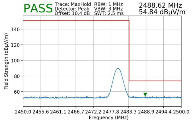
Plot 7-96. Radiated Restricted Upper Band Edge Measurement (Peak) – ANT 2
