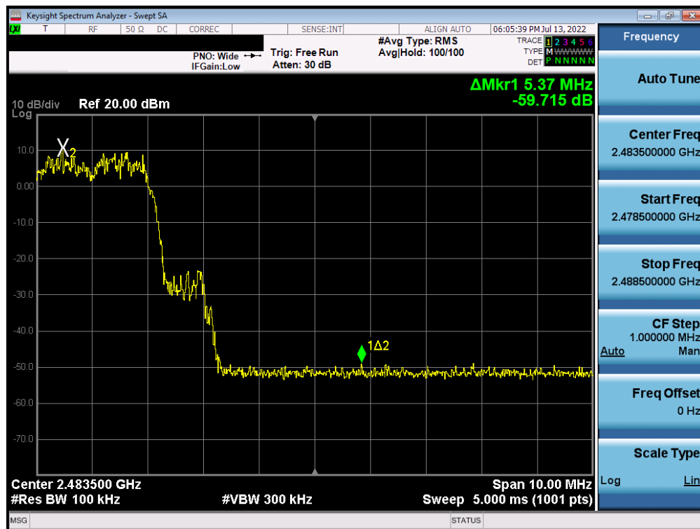
Plot 7-62. Band Edge Plot (Bluetooth with Hopping Enabled, 3 Mbps) – ANT 2
