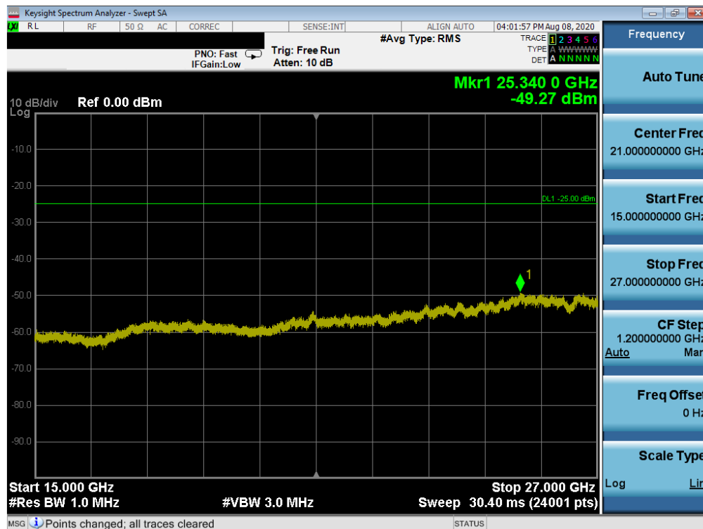
Plot 7-33. Conducted Spurious Plot (LTE Band 7 - 20MHz QPSK - RB Size 1, RB Offset 0 - High Channel)
