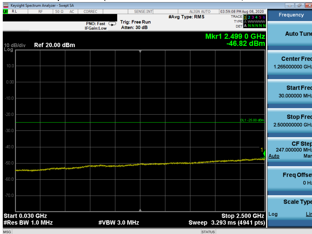
Plot 7-28. Conducted Spurious Plot (LTE Band 7 - 20MHz QPSK - RB Size 1, RB Offset 0 - Mid Channel)
