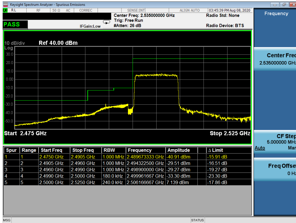
Plot 7-47. Lower ACP Plot (LTE Band 7 - 10MHz QPSK – Full RB Configuration)
