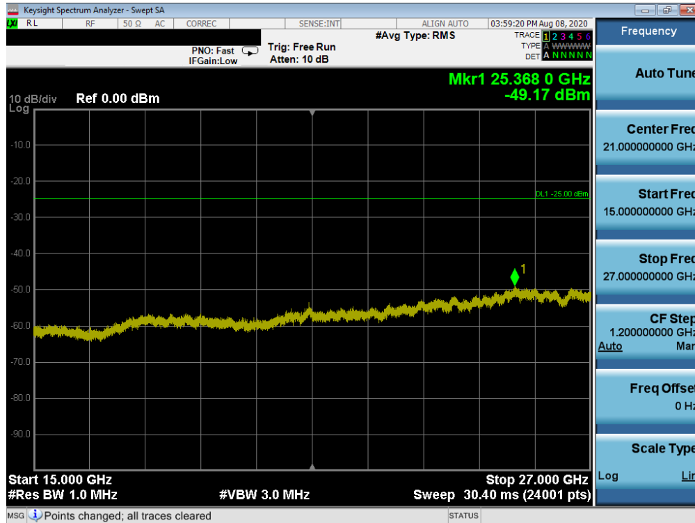
Plot 7-30. Conducted Spurious Plot (LTE Band 7 - 20MHz QPSK - RB Size 1, RB Offset 0 - Mid Channel)
