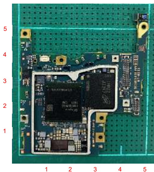
Internal Main-PWB Front without Shield cases (Front-side)
