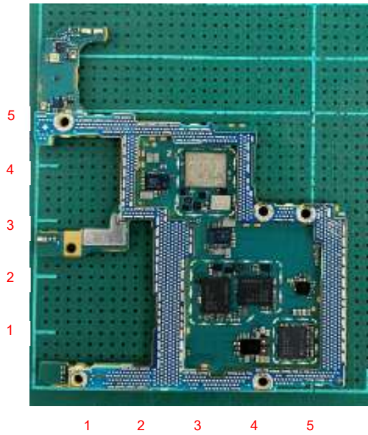
Internal Main-PWB Rear without Shield case (Front-side)
