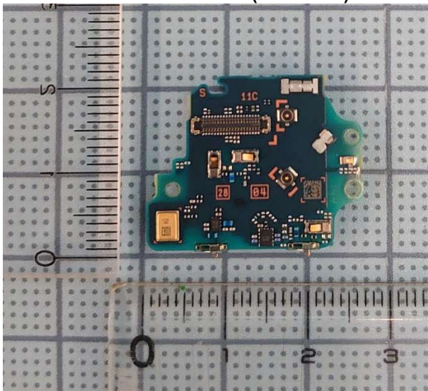
Internal Sub-PBA (Rear-side)
