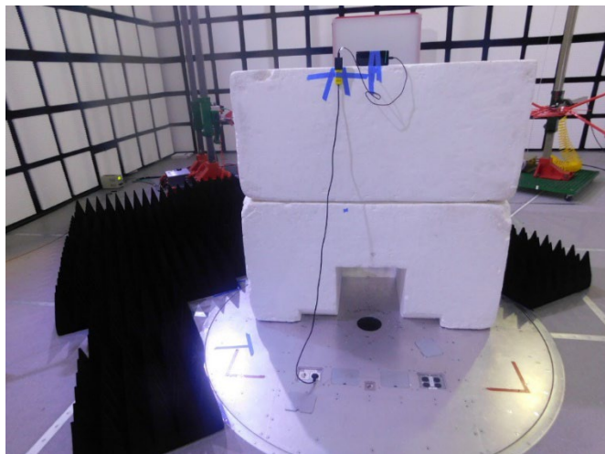
RADIATED EMISSIONS ABOVE 1GHz BACK
