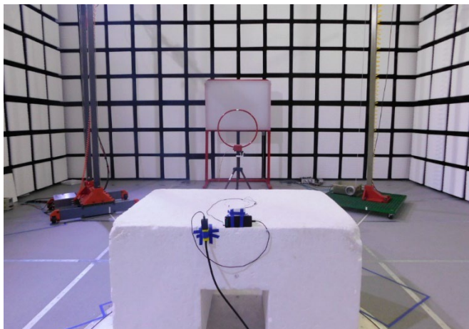
RADIATED EMISSIONS BELOW 30MHz 0Deg
