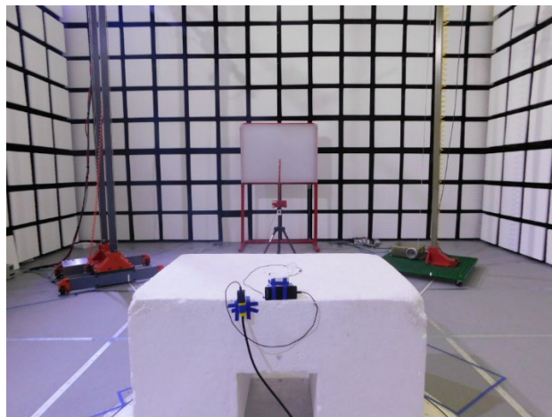
RADIATED EMISSIONS BELOW 30MHz 90Deg
