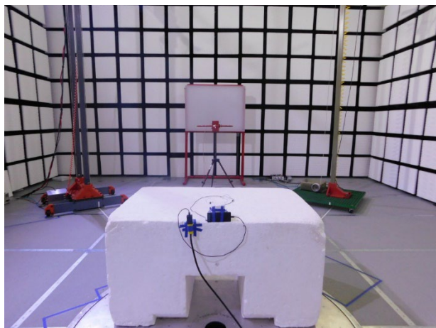
RADIATED EMISSIONS BELOW 30MHz FLAT
