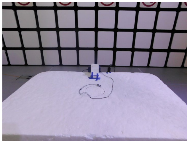
RADIATED EMISSIONS BELOW 30MHz BACK
