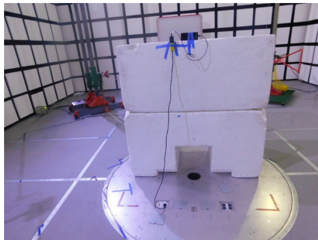
RADIATED EMISSIONS BELOW 1GHz FRONT
