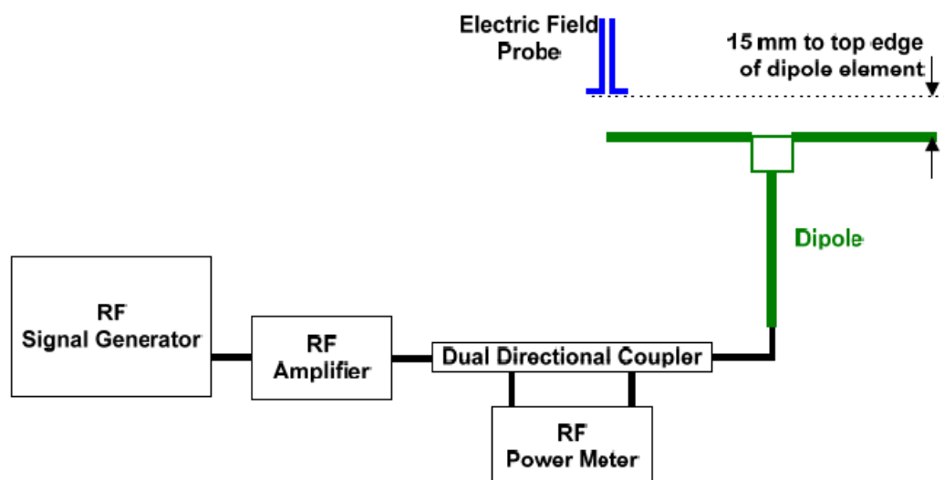
Fig. 7.1 Setup Diagram
