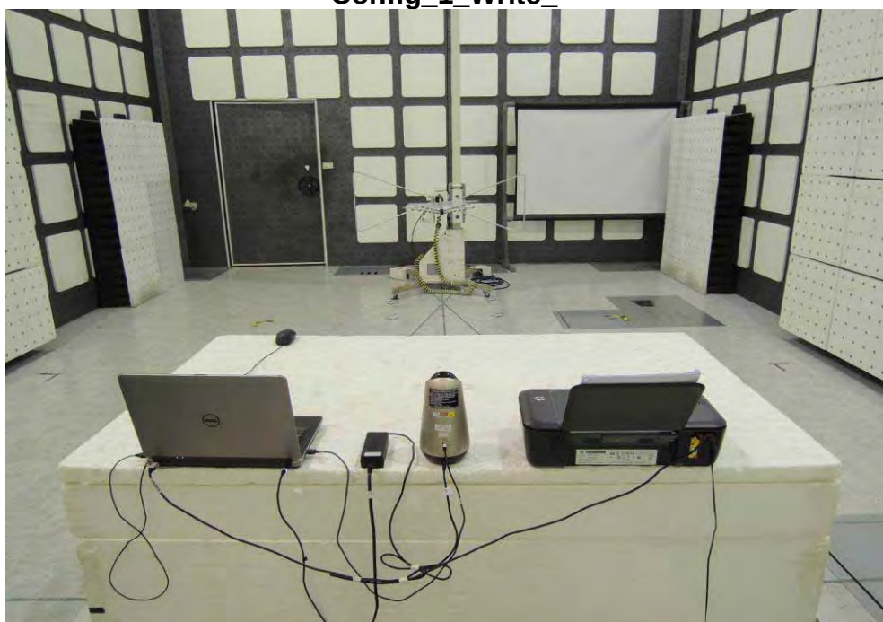
Config_1_Write_-
