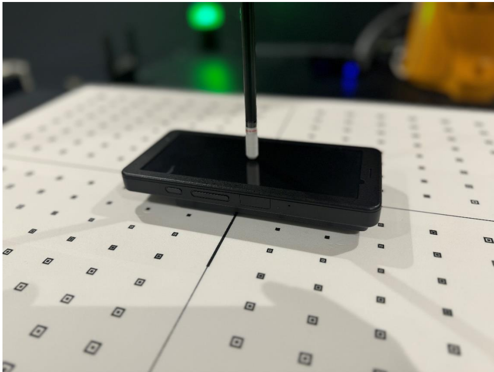
Figure M Power Density Test Setup – Body – Front 2mm
