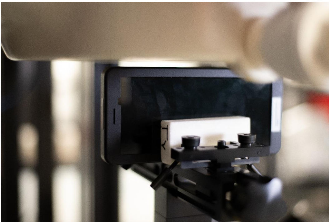
Figure J SAR Test Setup – Body – Right 5mm
