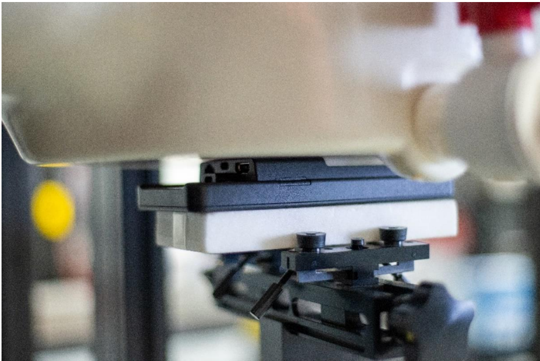
Figure B SAR Test Setup – Body – Back 0mm
