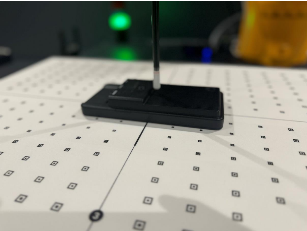
Figure L Power Density Test Setup – Body – Back 2mm
