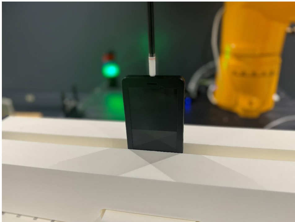
Figure N Power Density Test Setup – Body – Top 2mm
