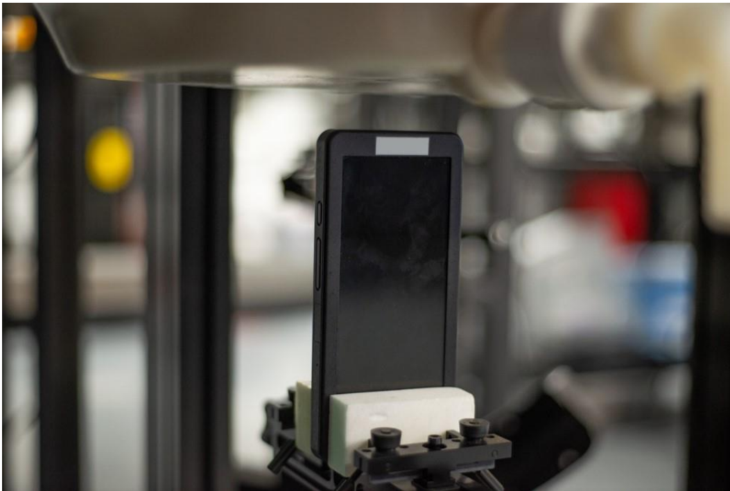
Figure I SAR Test Setup – Body – Bottom 25mm
