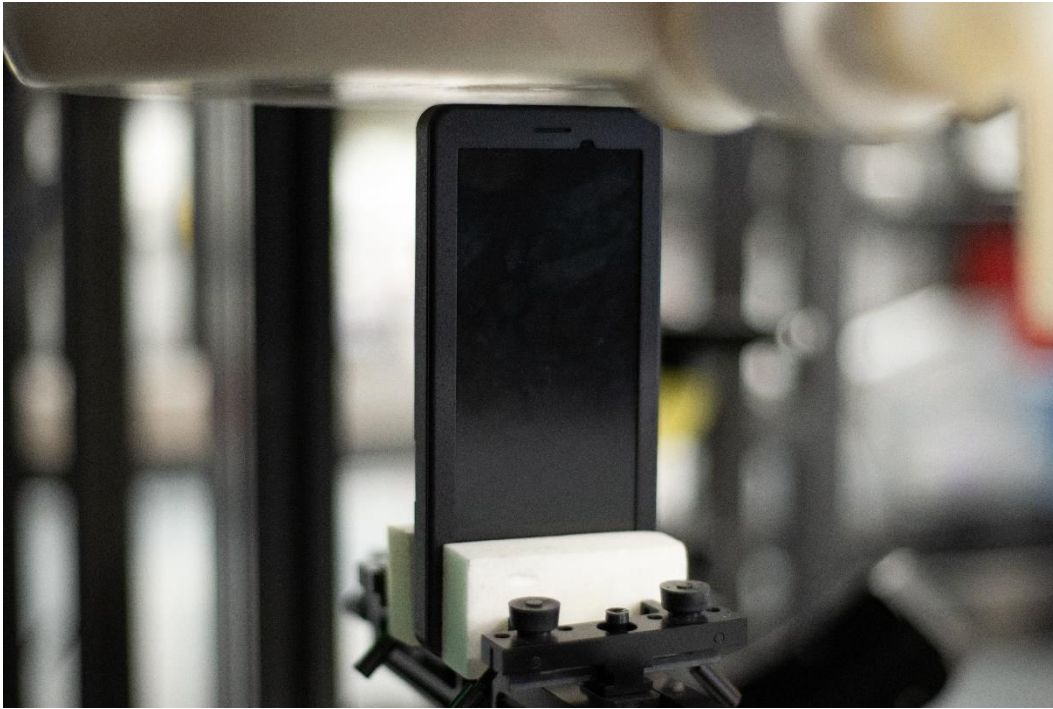
Figure E SAR Test Setup – Body – Top 5mm
