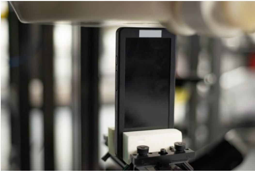
Figure G SAR Test Setup – Body – Bottom 5mm
