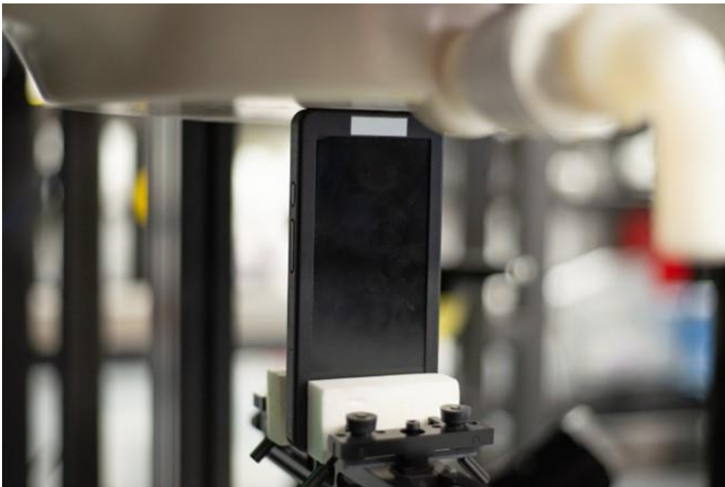
Figure H SAR Test Setup – Extremity – Bottom 0mm
