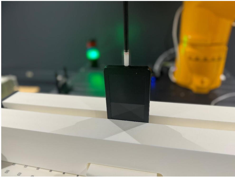
Figure O Power Density Test Setup – Body – Bottom 2mm
