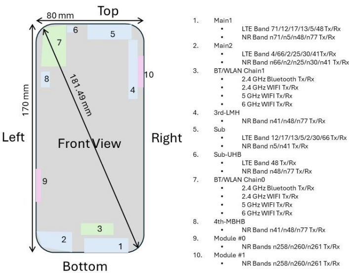
Figure A SAR Test Setup – Antenna Diagram
