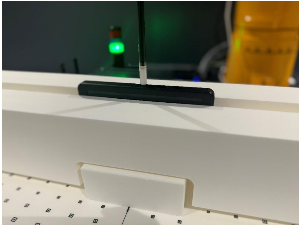
Figure P Power Density Test Setup – Body – Right 2mm
