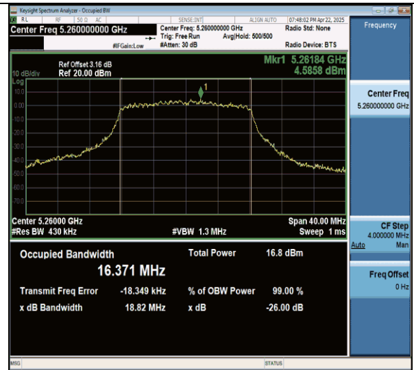
11a-CDD-Ant7-5260
