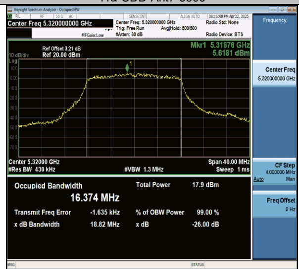
11a-CDD-Ant7-5320
