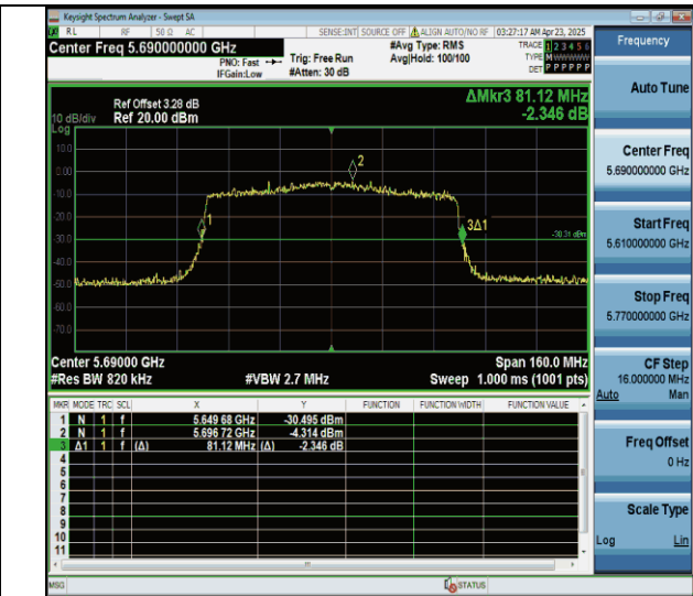
11ax80MIMO-Ant7-5690
