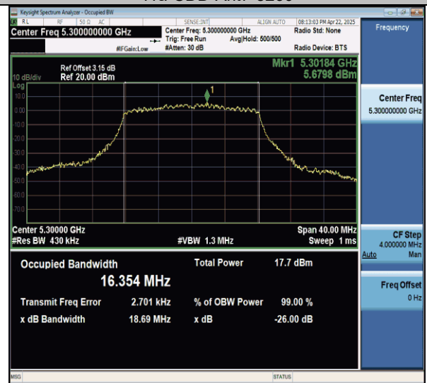
11a-CDD-Ant7-5300
