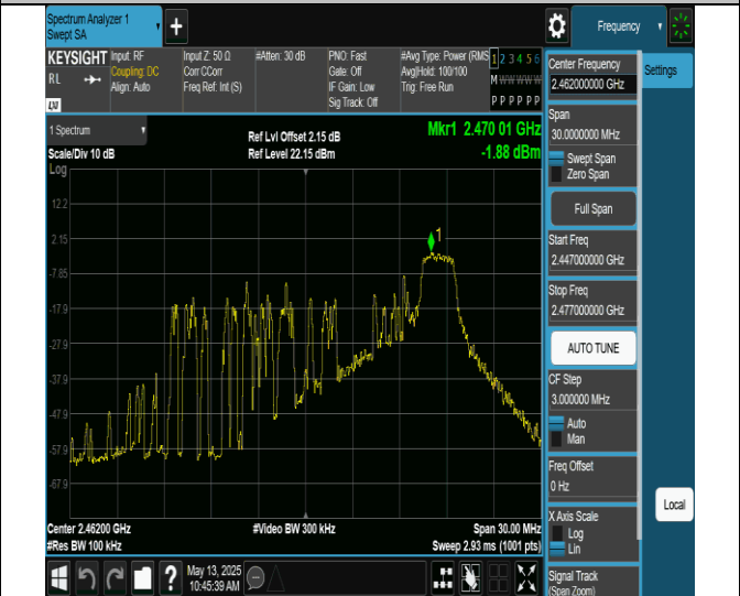
11ax20MIMO-Ant7-2462-26Tone-RU8-0~Reference-PASS
