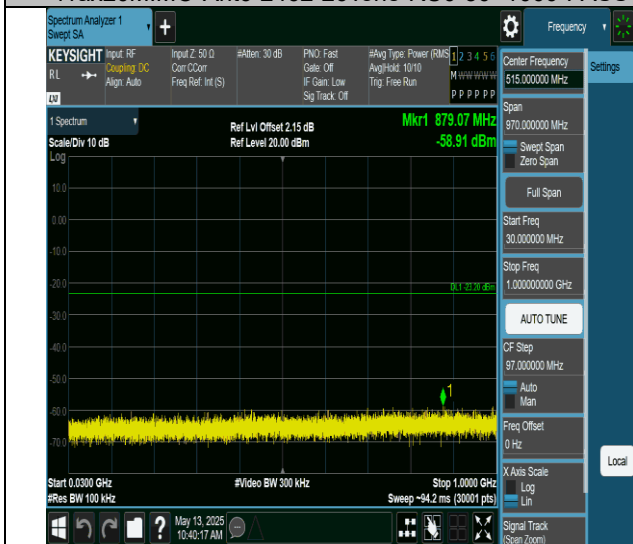
11ax20MIMO-Ant6-2462-26Tone-RU8-30~1000-PASS
