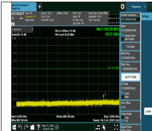
11ax20MIMO-Ant6-2462-26Tone-RU0-30~1000-PASS
