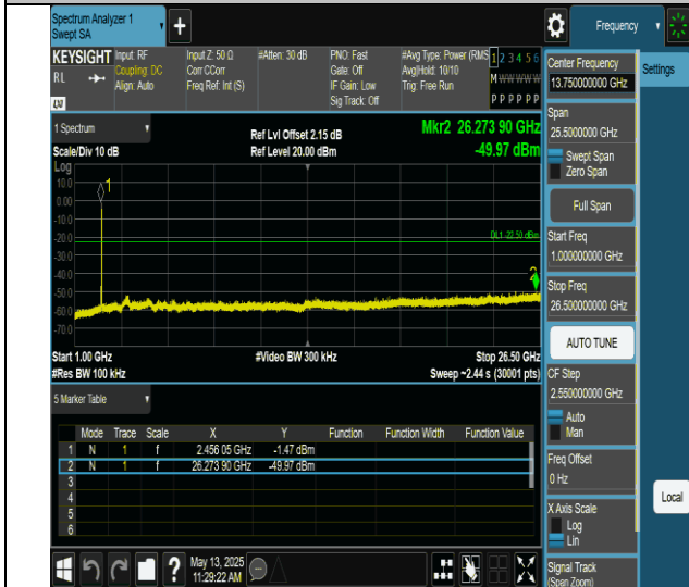
11ax20MIMO-Ant6-2462-106Tone-RU54-1000~26500-PASS
