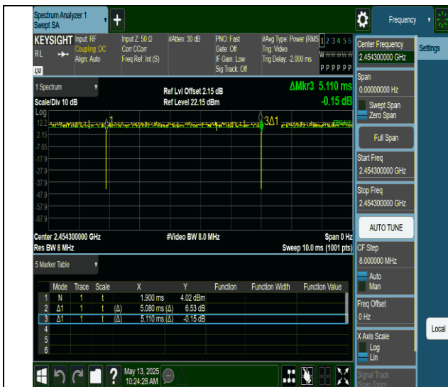
NTVN-11ax20MIMO-Ant6-2462-26Tone-RU0
