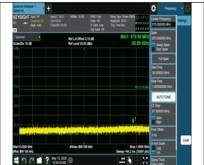
11ax20MIMO-Ant7-2462-26Tone-RU0-30~1000-PASS
