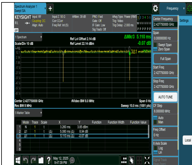
NTVN-11ax20MIMO-Ant6-2437-26Tone-RU0
