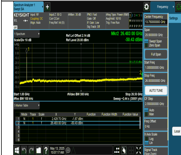
11ax20MIMO-Ant6-2437-106Tone-RU53-1000~26500-PASS
