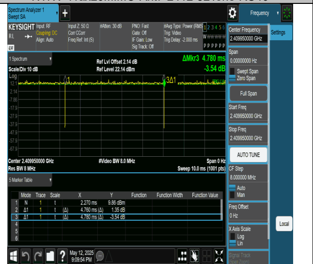
NTNV-11ax20MIMO-Ant7-2412-106Tone-RU53
