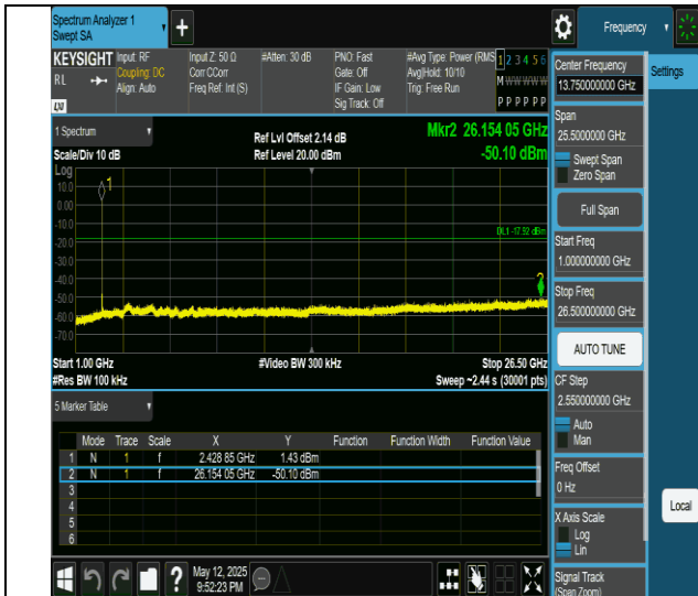
11ax20MIMO-Ant6-2437-26Tone-RU0-1000~26500-PASS
