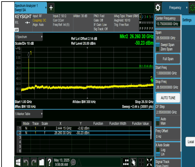
11ax20MIMO-Ant6-2437-52Tone-RU40-1000~26500-PASS
