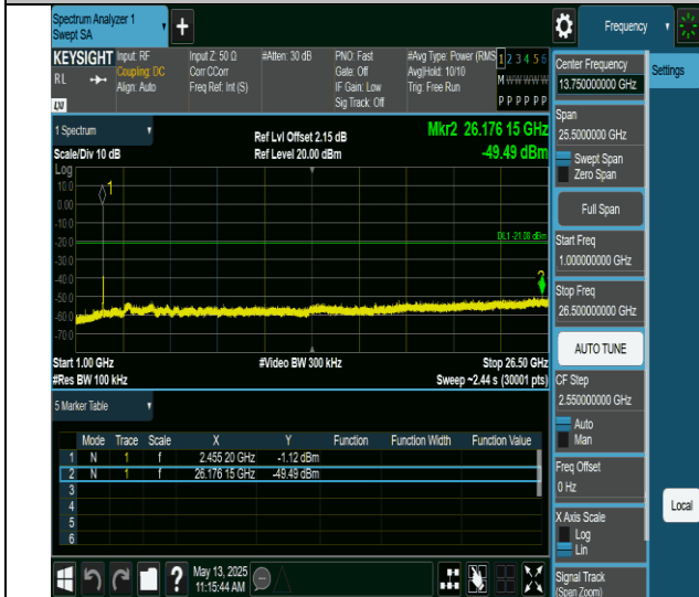
11ax20MIMO-Ant6-2462-106Tone-RU53-1000~26500-PASS
