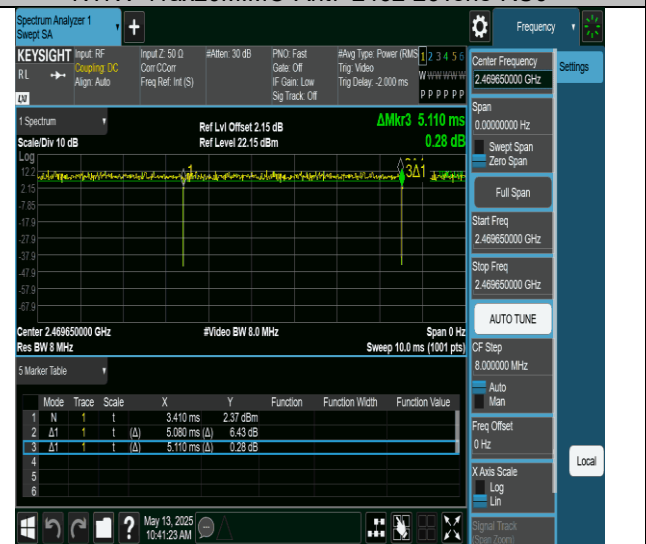
NTVN-11ax20MIMO-Ant7-2462-26Tone-RU8
