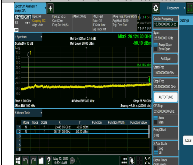
11ax20MIMO-Ant6-2437-26Tone-RU8-1000~26500-PASS
