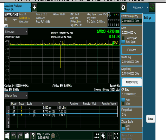
NTNV-11ax20MIMO-Ant7-2412-106Tone-RU54
