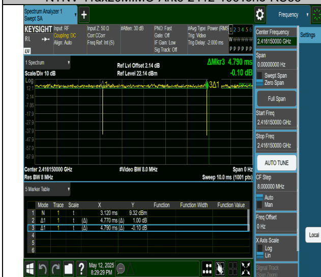
NTNV-11ax20MIMO-Ant6-2412-106Tone-RU54
