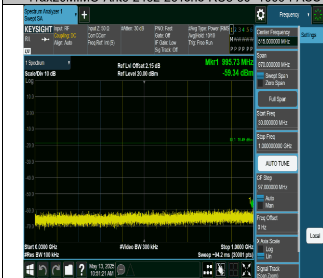
11ax20MIMO-Ant6-2462-52Tone-RU37-30~1000-PASS
