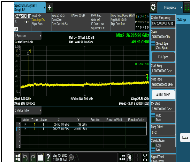
11ax20MIMO-Ant6-2462-52Tone-RU40-1000~26500-PASS
