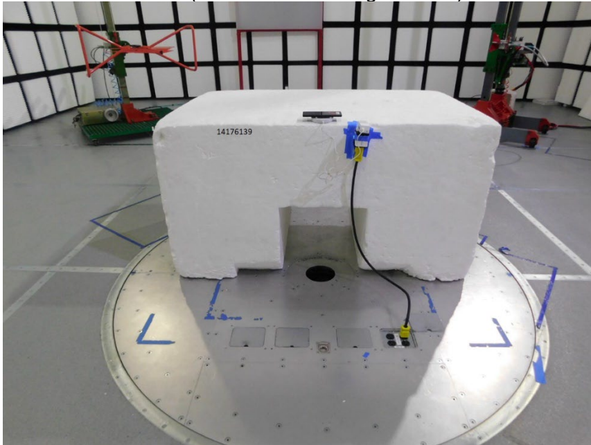
RADIATED PHOTO (30-1000MHz Configuration 3)
