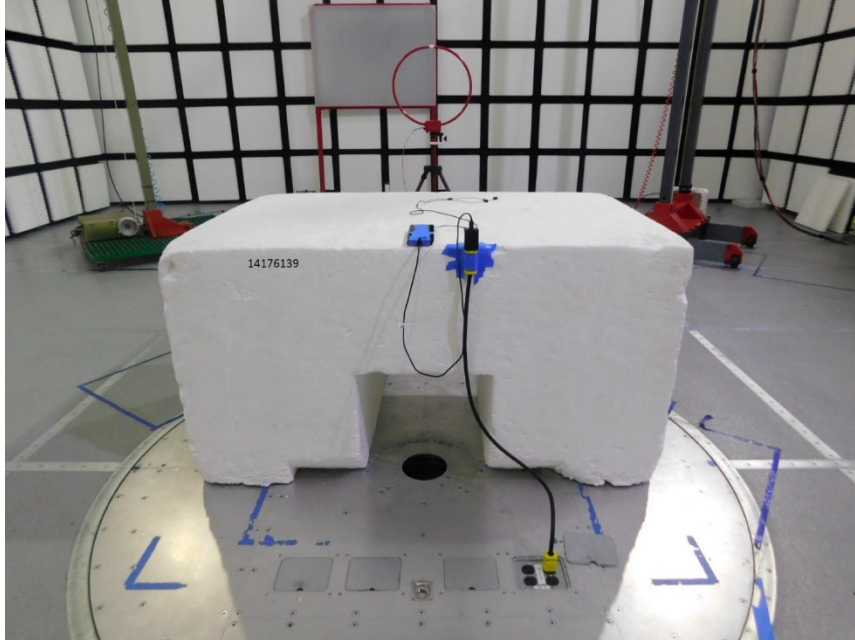
RADIATED PHOTO (<30 MHz WPT Configuration 1)
