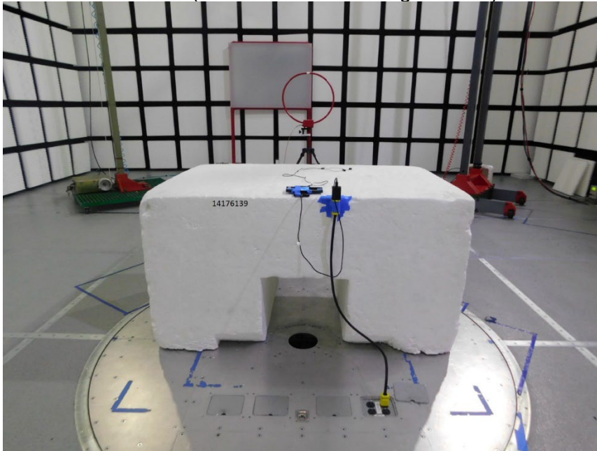
RADIATED PHOTO (<30 MHz WLAN Configuration 2)
