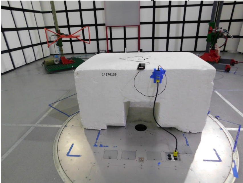
RADIATED PHOTO (30-1000MHz Configuration 1)
