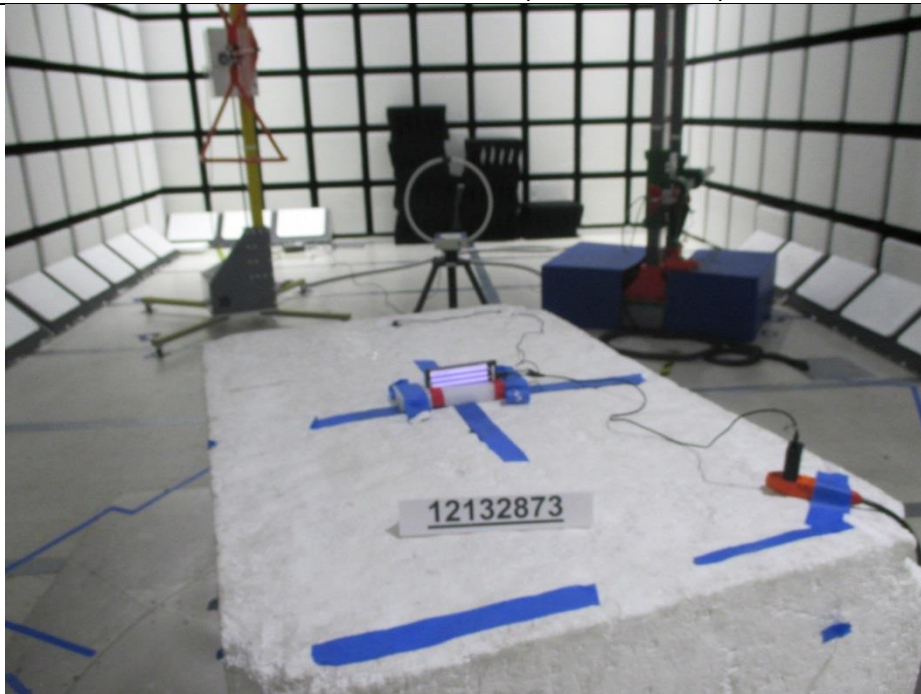
RADIATED BACK PHOTO (BELOW 30 MHz)
