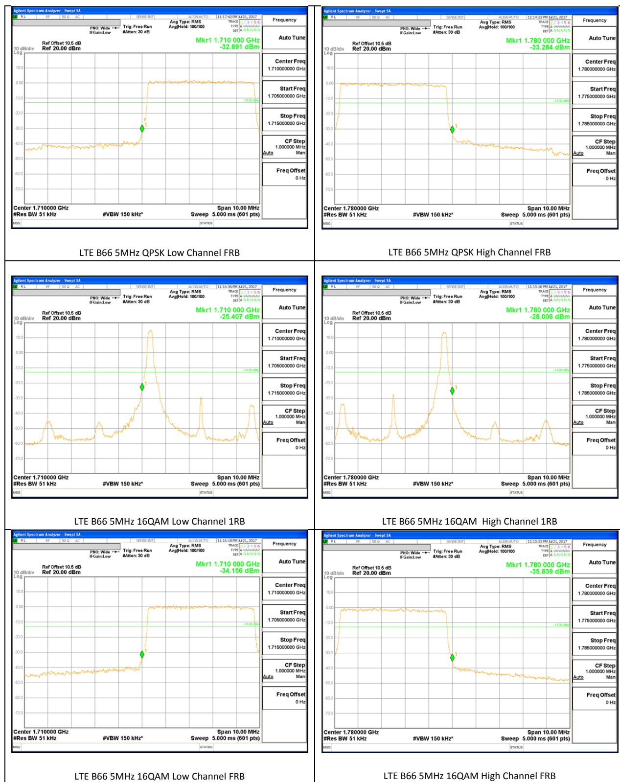
LTE B66 5MHz 16QAM Low Channel FRB
