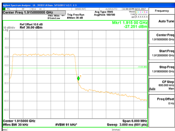
LTE B25 3MHz 16QAM High Channel FRB
