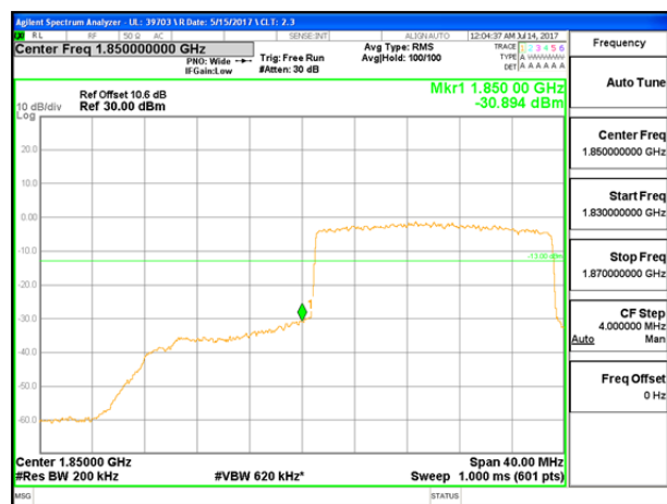
LTE B25 20MHz 16QAM Low Channel FRB
