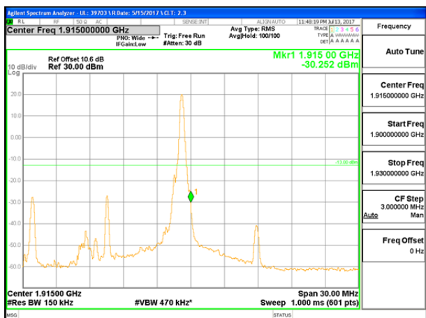
LTE B25 15MHz QPSK High Channel 1RB
