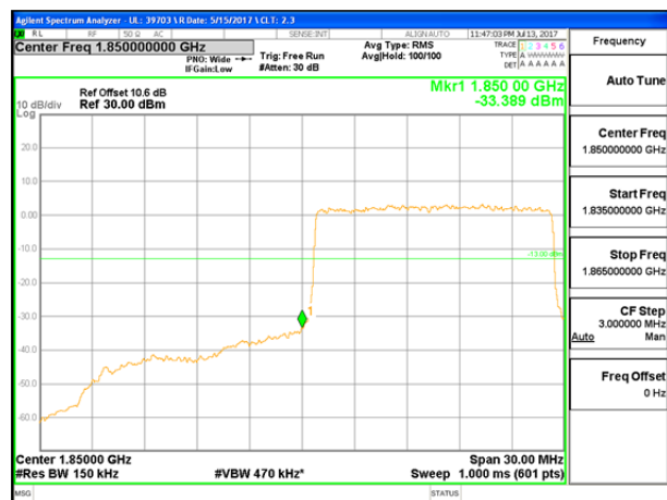
LTE B25 15MHz QPSK Low Channel FRB
