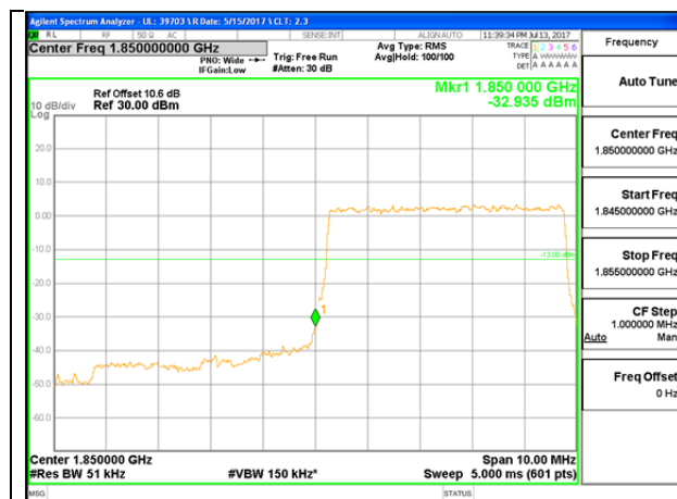
LTE B25 5MHz QPSK Low Channel FRB
