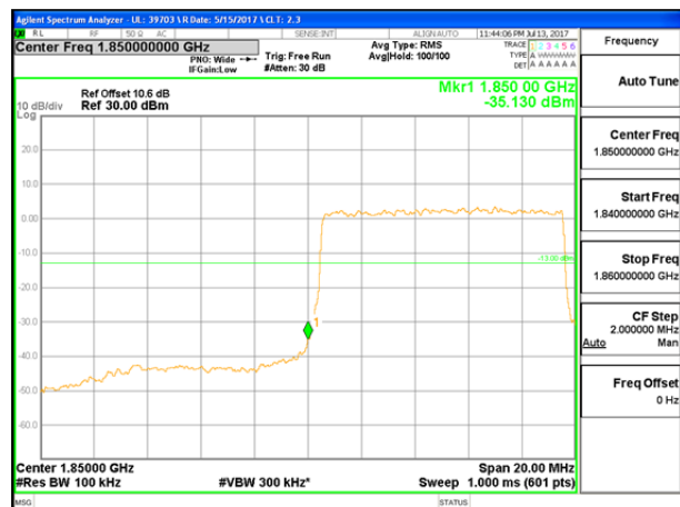
LTE B25 10MHz 16QAM Low Channel FRB
