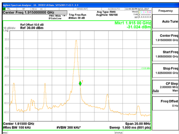
LTE B25 10MHz QPSK High Channel 1RB
