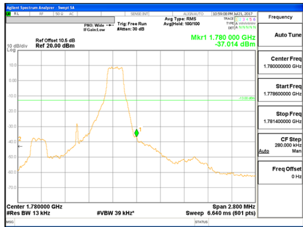
LTE B66 1.4MHz QPSK High Channel 1RB
