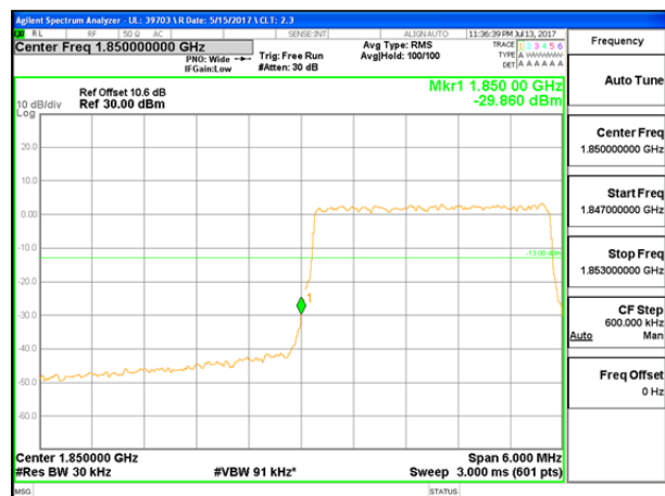
LTE B25 3MHz 16QAM Low Channel FRB
