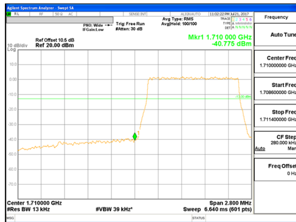
LTE B66 1.4MHz QPSK Low Channel FRB
