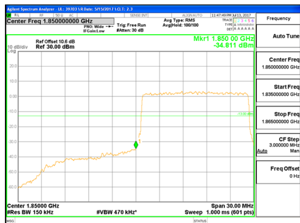
LTE B25 15MHz 16QAM Low Channel FRB
