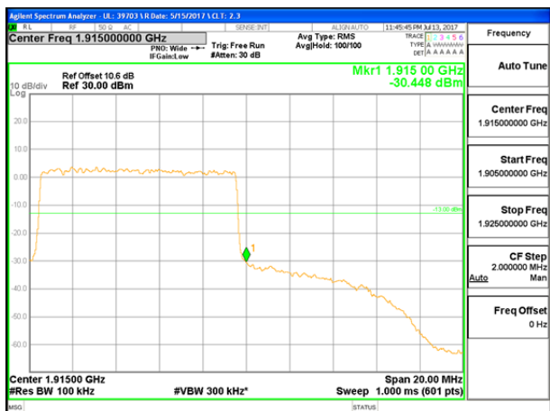
LTE B25 10MHz 16QAM High Channel FRB
