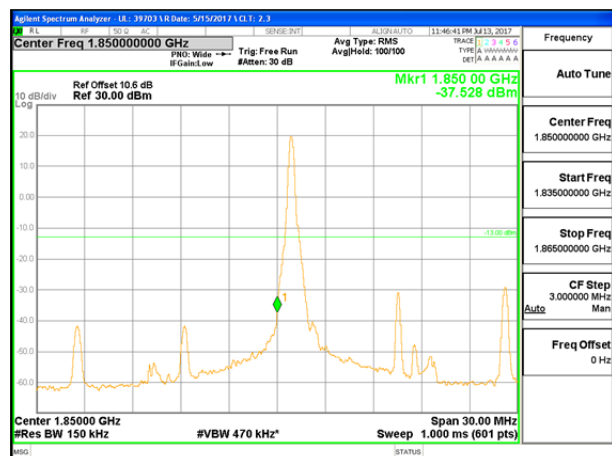
LTE B25 15MHz QPSK Low Channel 1RB
