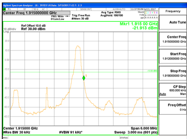
LTE B25 3MHz 16QAM High Channel 1RB
