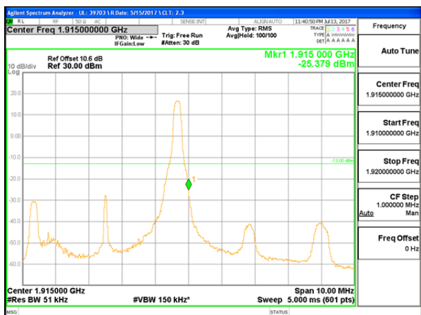
LTE B25 5MHz QPSK High Channel 1RB
