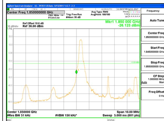
LTE B25 5MHz 16QAM Low Channel 1RB
