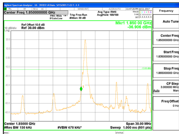
LTE B25 15MHz 16QAM Low Channel 1RB
