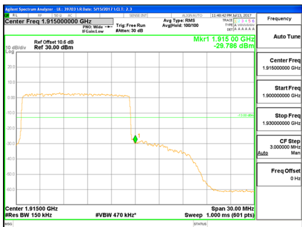
LTE B25 15MHz QPSK High Channel FRB
