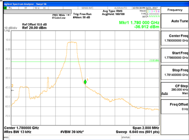
LTE B66 1.4MHz QPSK High Channel FRB
