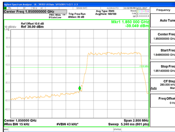
LTE B25 1.4MHz 16QAM Low Channel FRB
