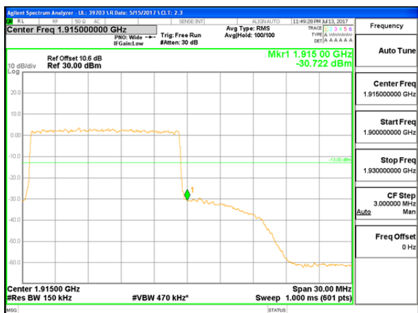
LTE B25 15MHz 16QAM High Channel FRB
