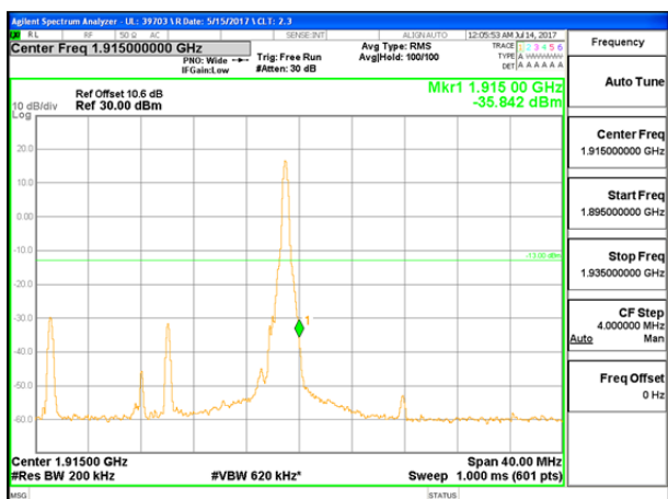
LTE B25 20MHz 16QAM High Channel 1RB
