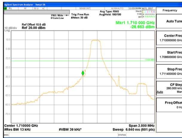
LTE B66 1.4MHz QPSK Low Channel 1RB
