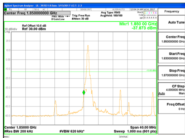
LTE B25 20MHz 16QAM Low Channel 1RB
