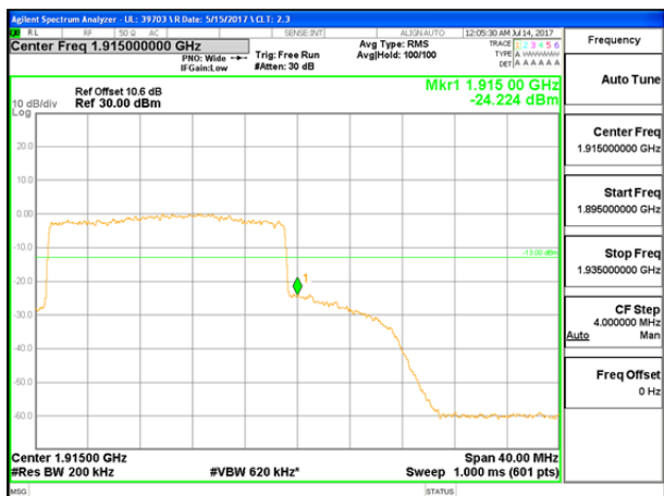
LTE B25 20MHz QPSK High Channel FRB
