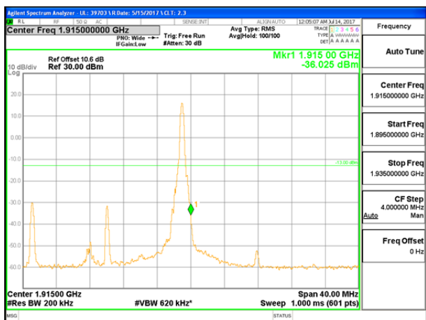
LTE B25 20MHz QPSK High Channel 1RB
