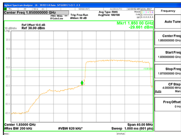
LTE B25 20MHz QPSK Low Channel FRB
