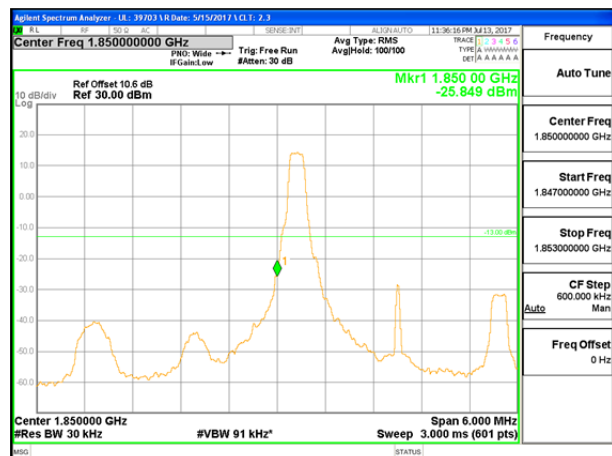
LTE B25 3MHz 16QAM Low Channel 1RB
