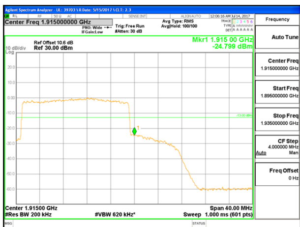
LTE B25 20MHz 16QAM High Channel FRB
