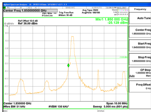
LTE B25 5MHz QPSK Low Channel 1RB
