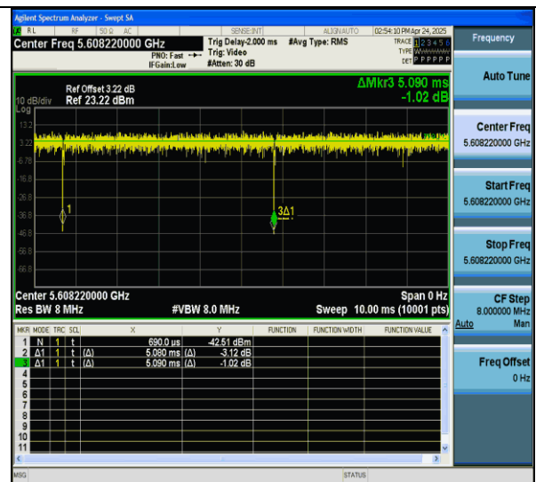
NTNV-11ax20MIMO-Ant7-5600-52Tone-RU40
