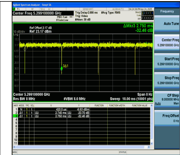
NTNV-11ax40MIMO-Ant7-5310-242Tone-RU61
