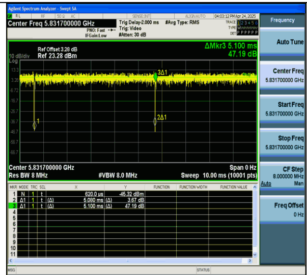
NTNV-11ax20MIMO-Ant7-5825-52Tone-RU40
