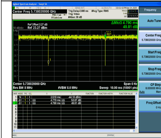
NTNV-11ax20MIMO-Ant6-5745-106Tone-RU53
