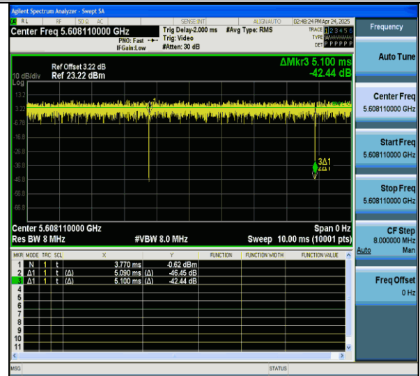
NTVN-11ax20MIMO-Ant7-5600-26Tone-RU8
