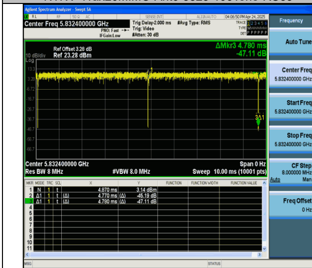
NTNV-11ax20MIMO-Ant6-5825-106Tone-RU54
