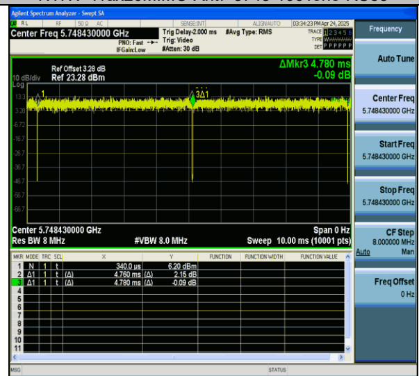
NTNV-11ax20MIMO-Ant7-5745-106Tone-RU54
