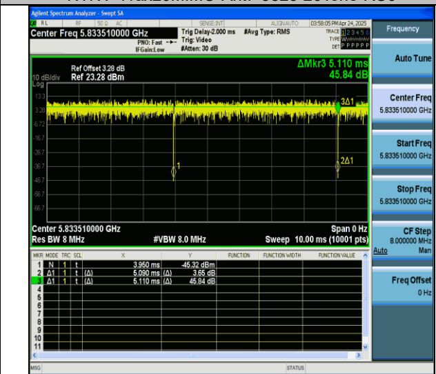
NTVN-11ax20MIMO-Ant7-5825-26Tone-RU8
