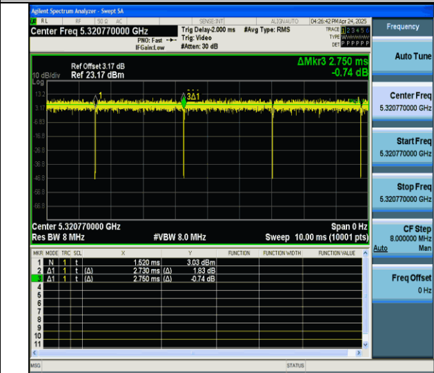
NTNV-11ax40MIMO-Ant7-5310-242Tone-RU62
