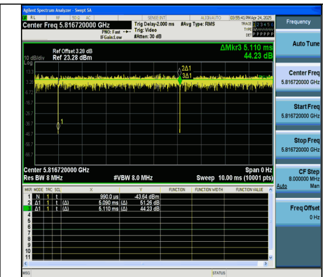
NTVN-11ax20MIMO-Ant7-5825-26Tone-RU0
