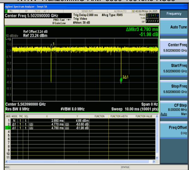
NTNV-11ax20MIMO-Ant7-5500-106Tone-RU54
