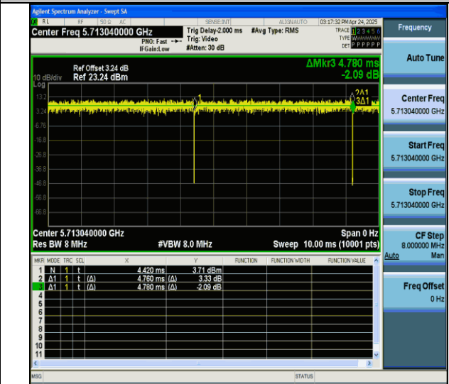
NTNV-11ax20MIMO-Ant7-5720-106Tone-RU53
