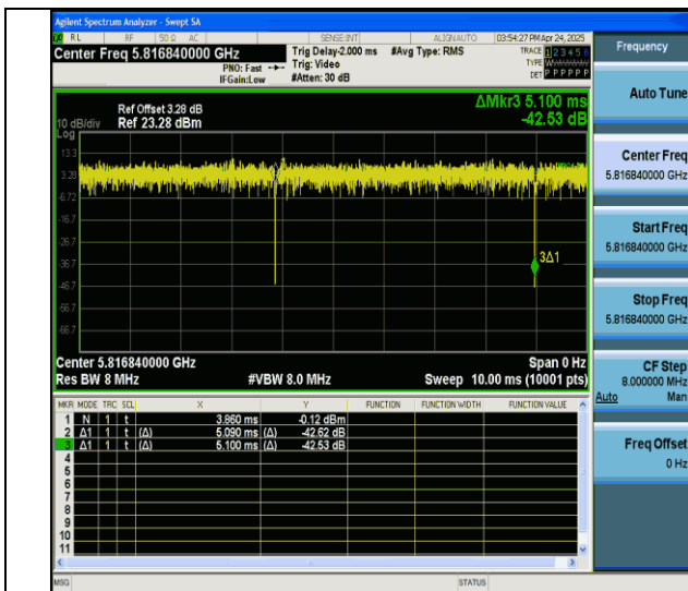
NTVN-11ax20MIMO-Ant6-5825-26Tone-RU0
