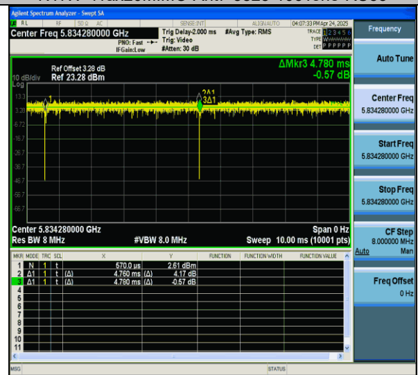
NTNV-11ax20MIMO-Ant7-5825-106Tone-RU54
