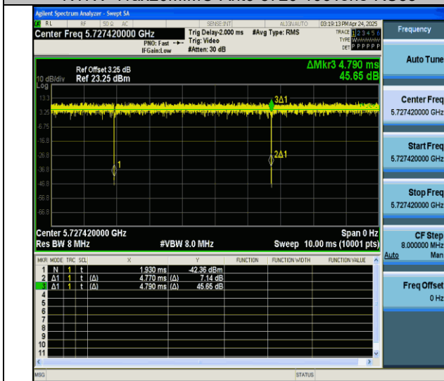
NTNV-11ax20MIMO-Ant6-5720-106Tone-RU54
