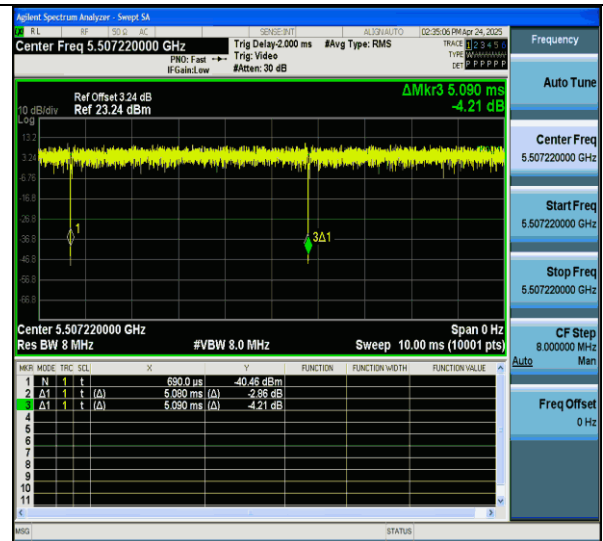
NTNV-11ax20MIMO-Ant7-5500-52Tone-RU40
