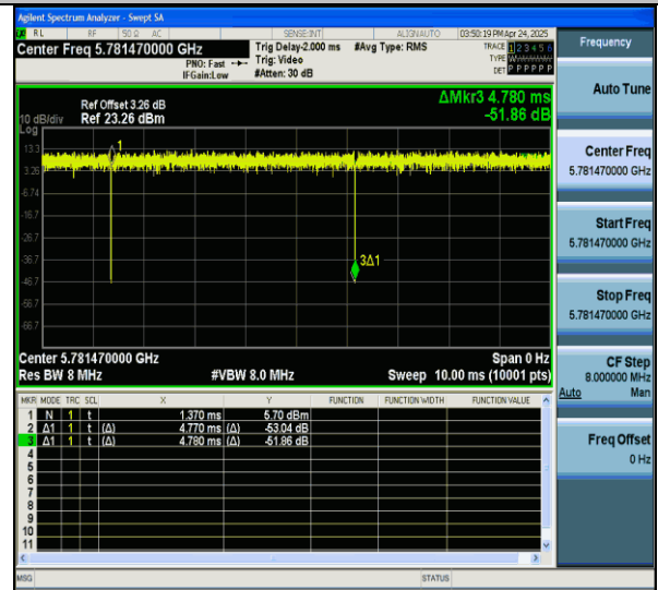
NTNV-11ax20MIMO-Ant7-5785-106Tone-RU53
