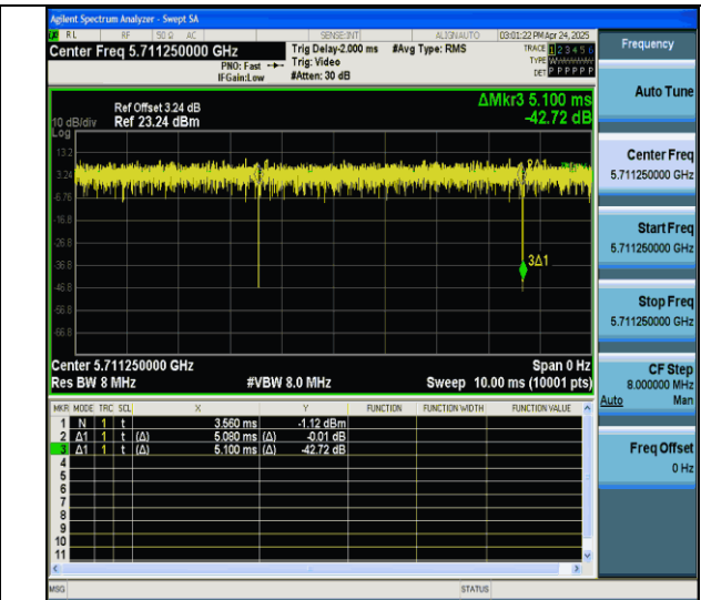
NTVN-11ax20MIMO-Ant7-5720-26Tone-RU0
