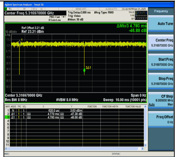
NTNV-11ax20MIMO-Ant7-5320-106Tone-RU53
