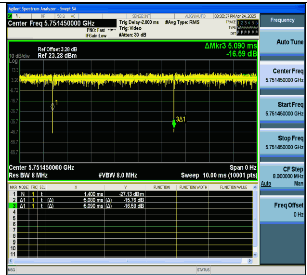
NTNV-11ax20MIMO-Ant7-5745-52Tone-RU40
