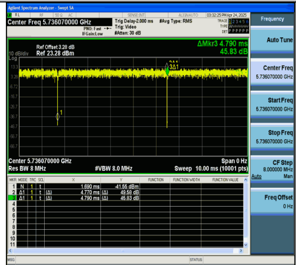
NTNV-11ax20MIMO-Ant7-5745-106Tone-RU53
