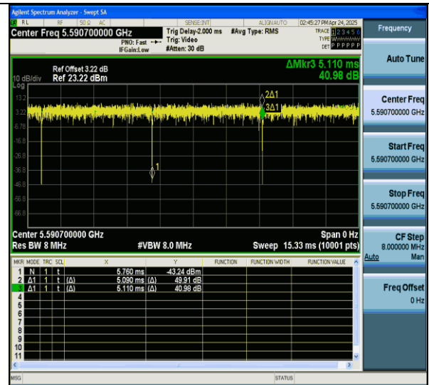
NTVN-11ax20MIMO-Ant7-5600-26Tone-RU0
