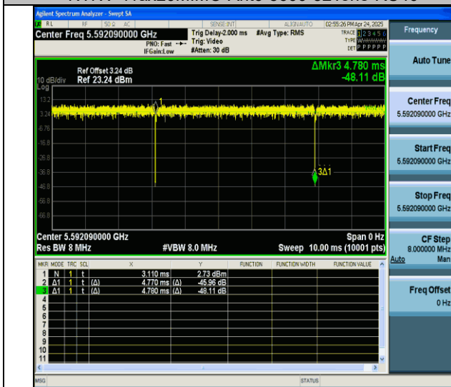
NTNV-11ax20MIMO-Ant6-5600-106Tone-RU53
