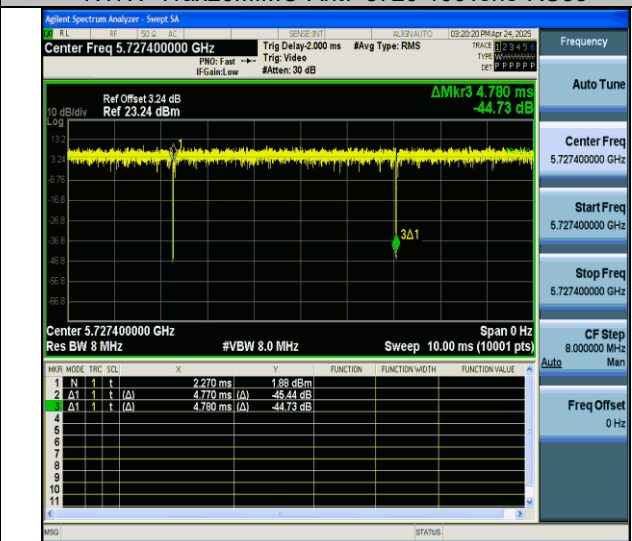
NTNV-11ax20MIMO-Ant7-5720-106Tone-RU54
