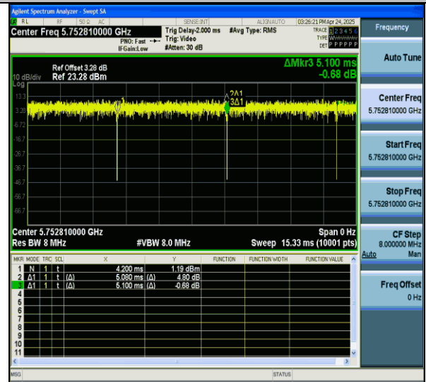
NTVN-11ax20MIMO-Ant7-5745-26Tone-RU8
