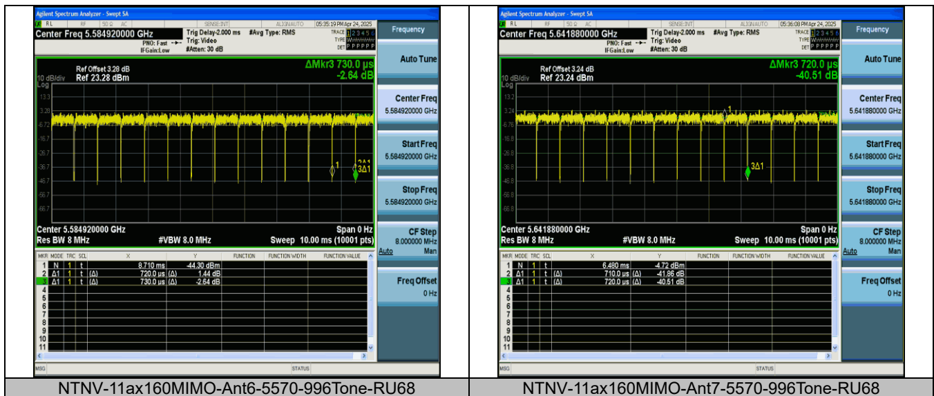
NTNV-11ax160MIMO-Ant6-5570-996Tone-RU68
