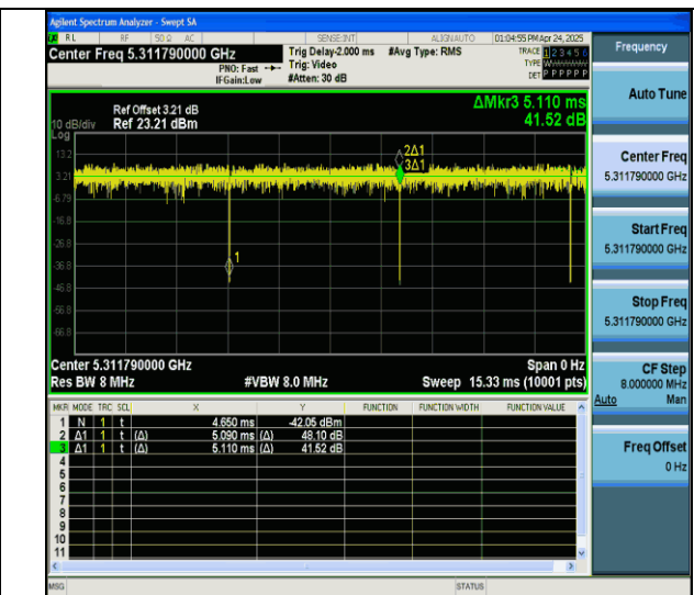
NTVN-11ax20MIMO-Ant7-5320-26Tone-RU0
