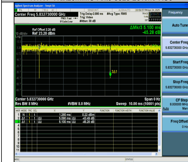
NTVN-11ax20MIMO-Ant6-5825-26Tone-RU8
