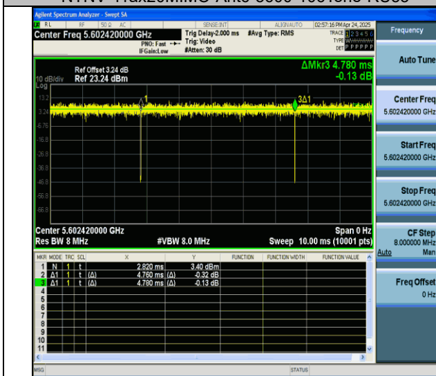
NTNV-11ax20MIMO-Ant6-5600-106Tone-RU54
