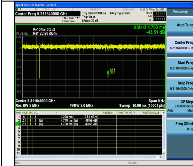
NTNV-11ax20MIMO-Ant6-5320-106Tone-RU53
