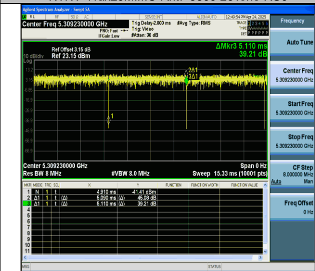
NTVN-11ax20MIMO-Ant7-5300-26Tone-RU8
