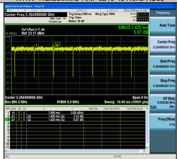
NTNV-11ax80MIMO-Ant7-5290-484Tone-RU65
