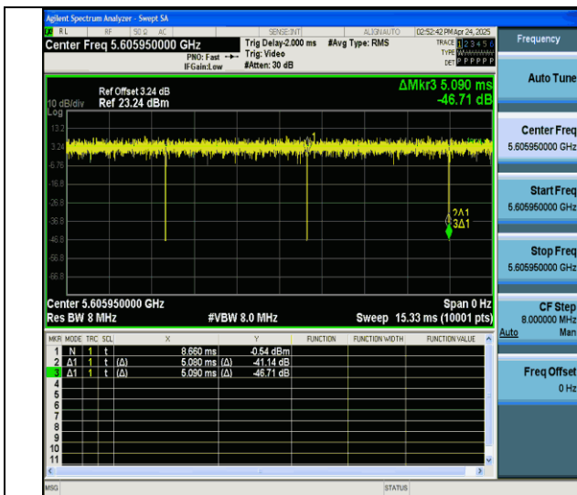
NTNV-11ax20MIMO-Ant6-5600-52Tone-RU40
