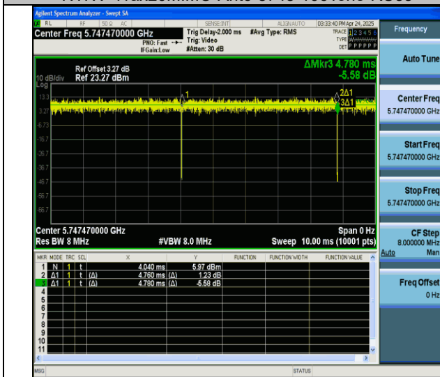
NTNV-11ax20MIMO-Ant6-5745-106Tone-RU54
