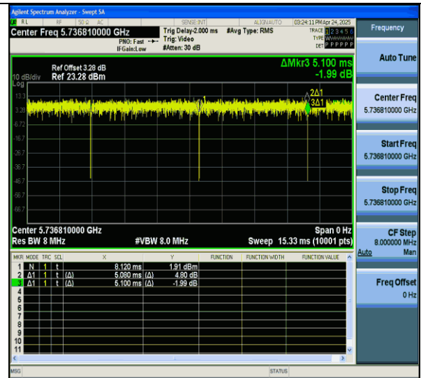
NTVN-11ax20MIMO-Ant7-5745-26Tone-RU0
