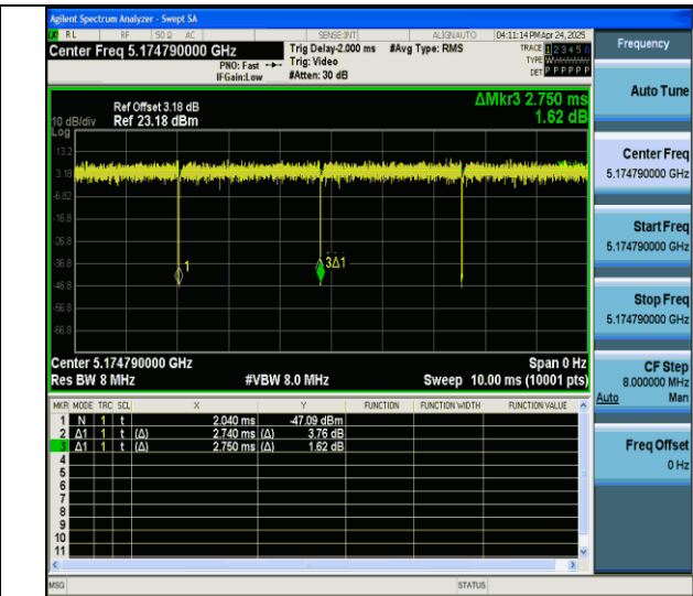
NTNV-11ax40MIMO-Ant7-5190-242Tone-RU61
