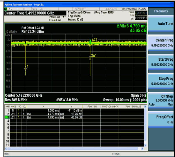
NTNV-11ax20MIMO-Ant7-5500-106Tone-RU53
