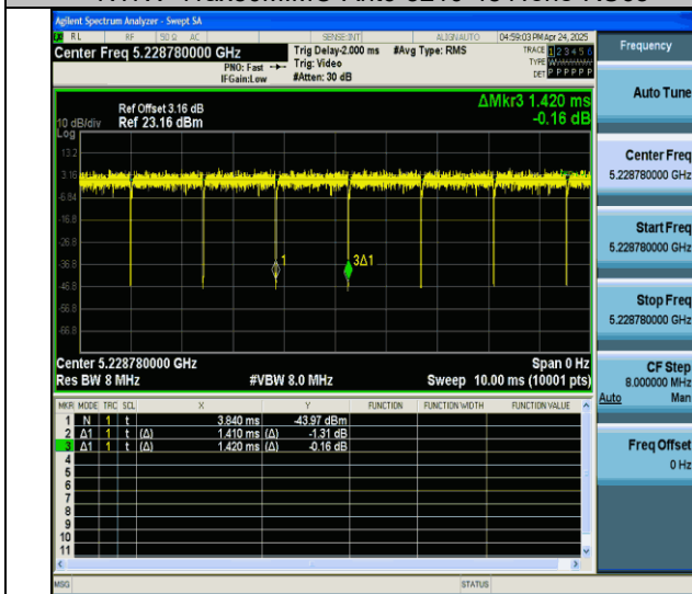
NTNV-11ax80MIMO-Ant6-5210-484Tone-RU66
