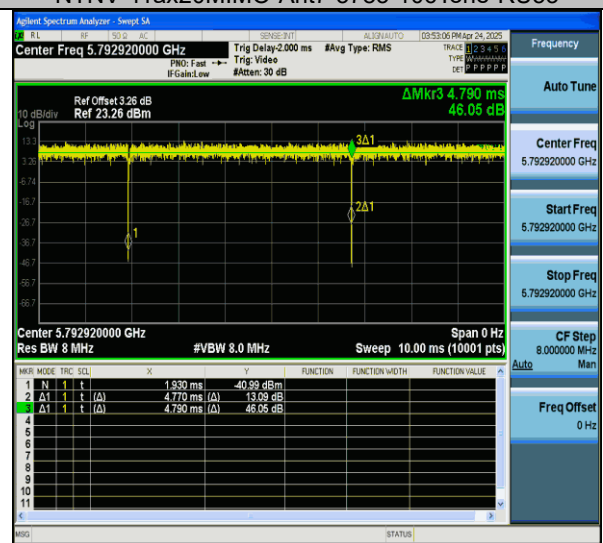
NTNV-11ax20MIMO-Ant7-5785-106Tone-RU54
