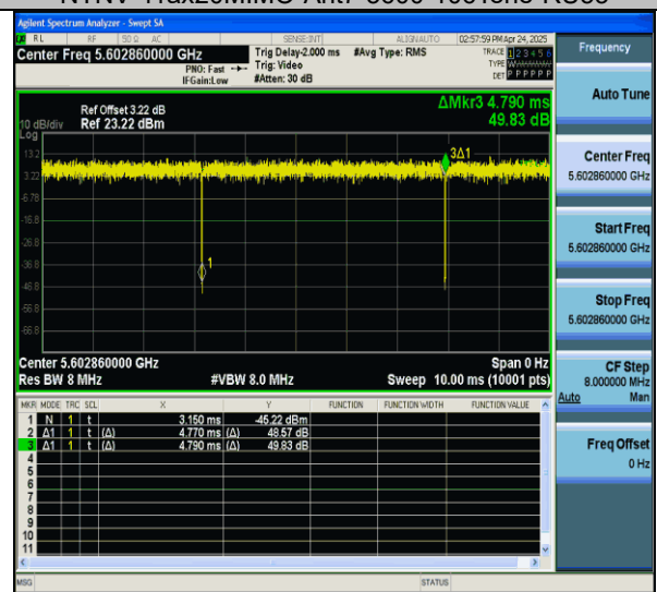
NTNV-11ax20MIMO-Ant7-5600-106Tone-RU54
