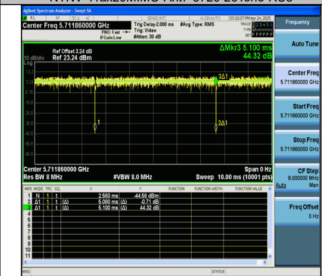
NTVN-11ax20MIMO-Ant7-5720-52Tone-RU37
