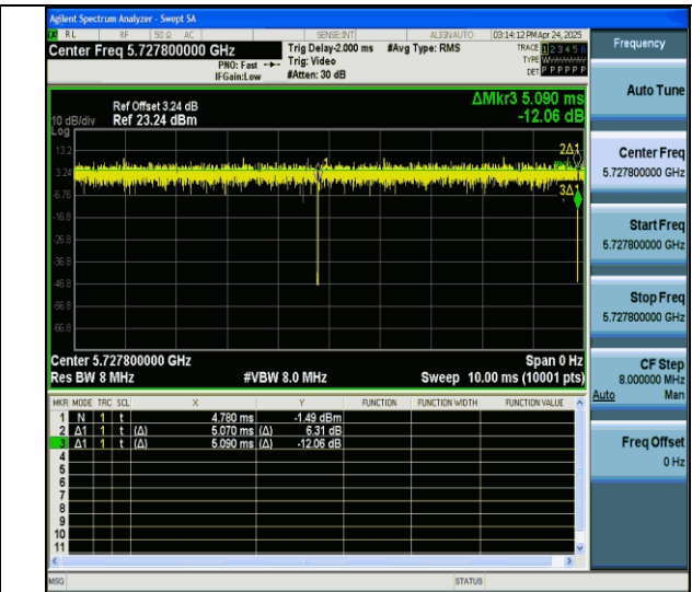
NTNV-11ax20MIMO-Ant7-5720-52Tone-RU40
