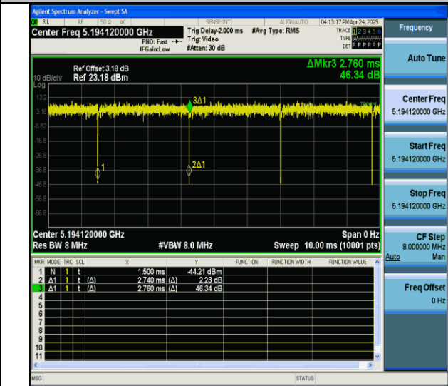
NTNV-11ax40MIMO-Ant7-5190-242Tone-RU62
