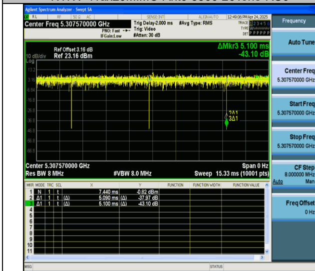
NTVN-11ax20MIMO-Ant6-5300-26Tone-RU8
