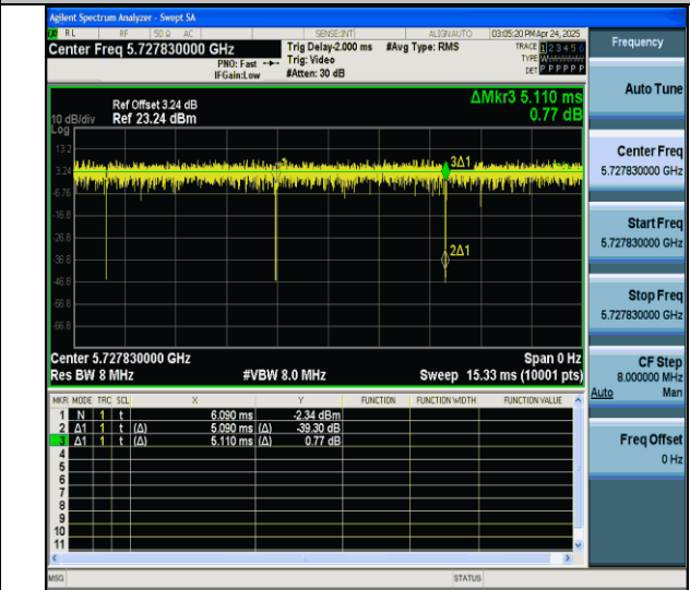
NTVN-11ax20MIMO-Ant7-5720-26Tone-RU8
