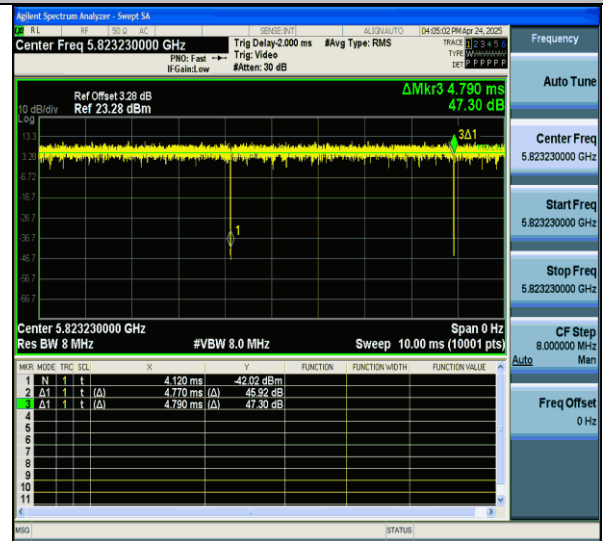
NTNV-11ax20MIMO-Ant7-5825-106Tone-RU53
