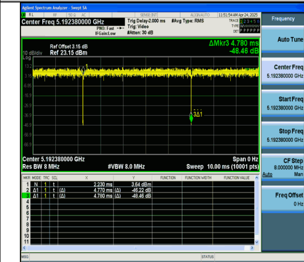
NTNV-11ax20MIMO-Ant7-5200-106Tone-RU53
