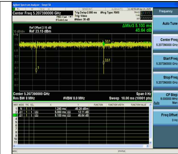
NTNV-11ax20MIMO-Ant7-5200-52Tone-RU40
