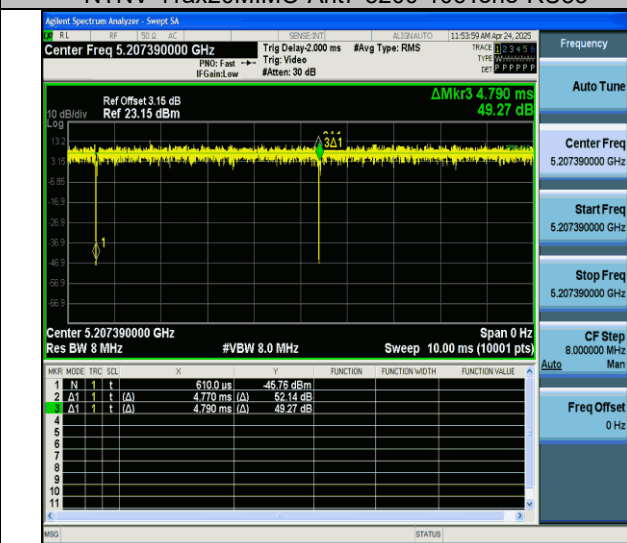
NTNV-11ax20MIMO-Ant7-5200-106Tone-RU54
