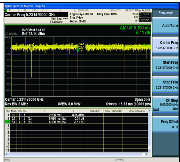
NTVN-11ax20MIMO-Ant7-5240-26Tone-RU0
