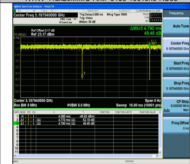
NTNV-11ax20MIMO-Ant7-5180-106Tone-RU54
