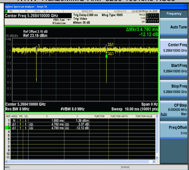
NTVN-11ax20MIMO-Ant7-5260-106Tone-RU54
