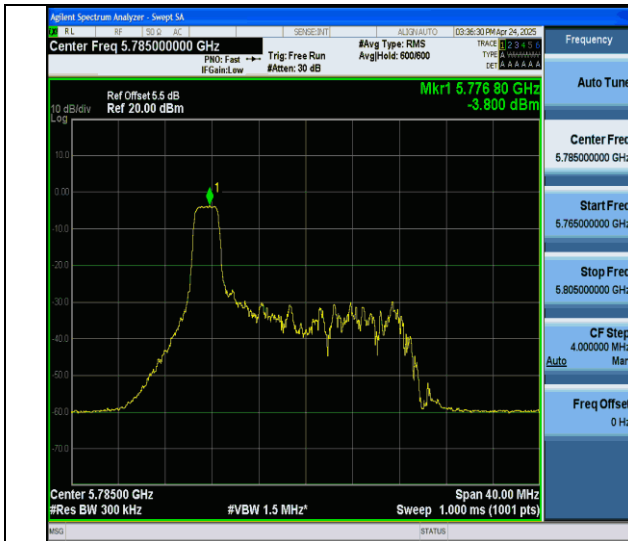
11ax20MIMO-Ant6-5785-26Tone-RU0-PASS
