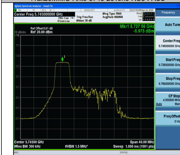
11ax20MIMO-Ant6-5745-52Tone-RU37-PASS
