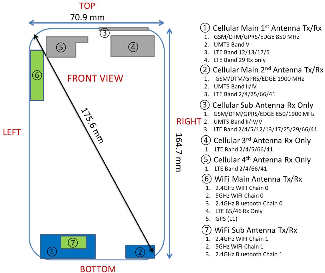
Figure J-1 DUT Antenna Locations
