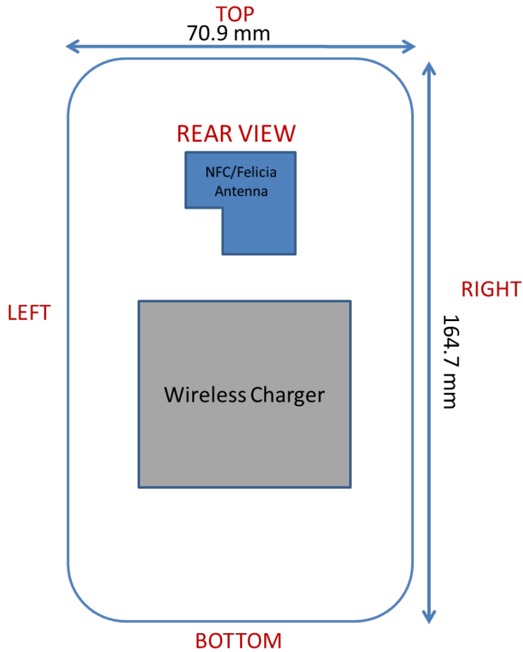
Figure J-2 NFC Antenna Locations
