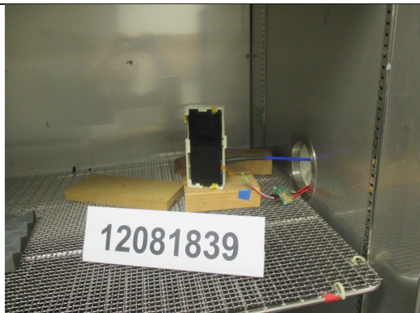
FREQUENCY STABILITY
