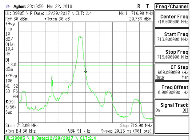
LTE B12 3MHz QPSK High Channel RB1-14
