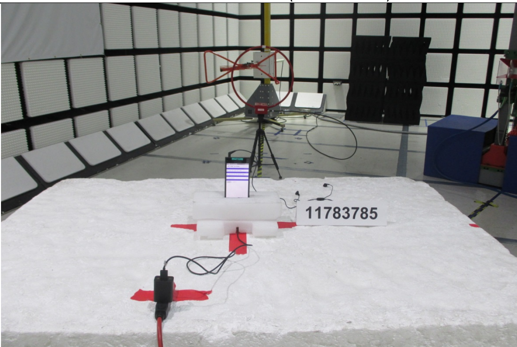
RADIATED BACK PHOTO (BELOW 30 MHz)
