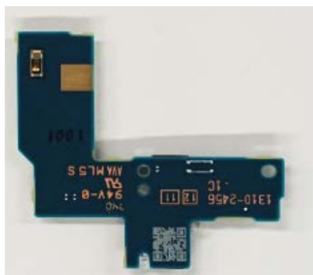
Internal Sub-PWB (Rear-side)
