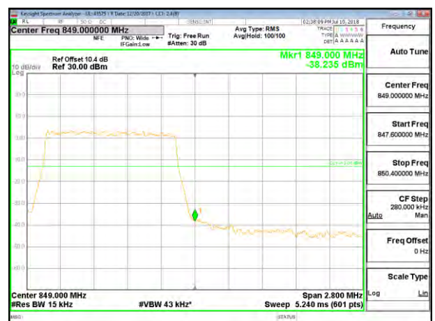
LTE B5 1.4MHz QPSK High Channel RB6-0
