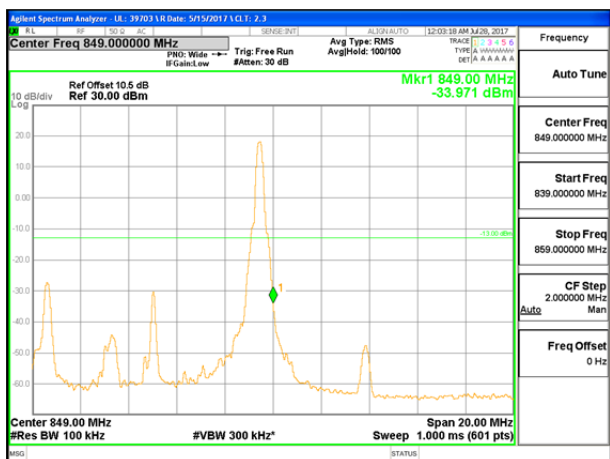
LTE B5 10MHz 16QAM High Channel 1RB
