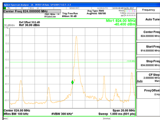
LTE B5 10MHz 16QAM Low Channel 1RB
