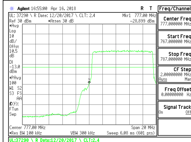
LTE B13 10MHz QPSK Low Channel RB50-0
