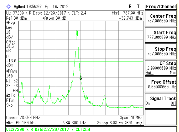
LTE B13 10MHz QPSK High Channel RB1-0
