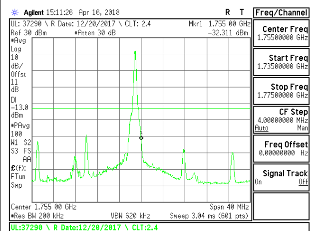
LTE B4 20MHz 16QAM High Channel RB1-0
