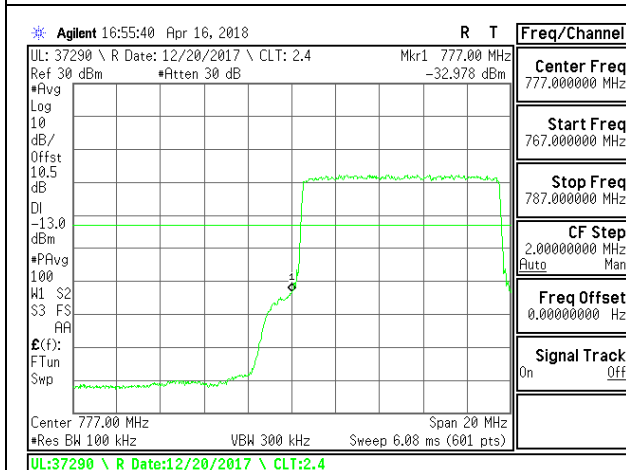
LTE B13 10MHz 16QAM Low Channel RB50-0
