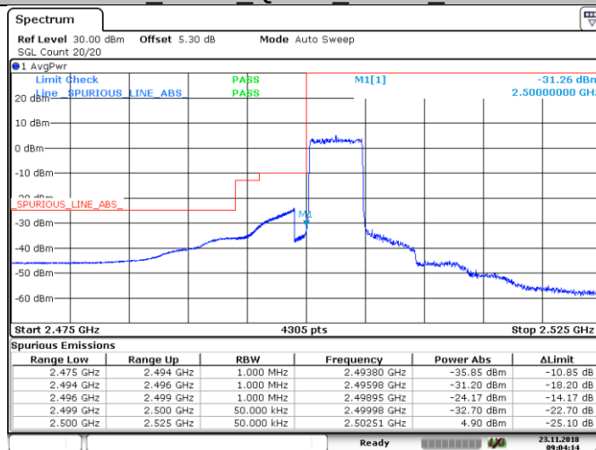
Band7_5MHz_QPSK_20775_25RB#0
