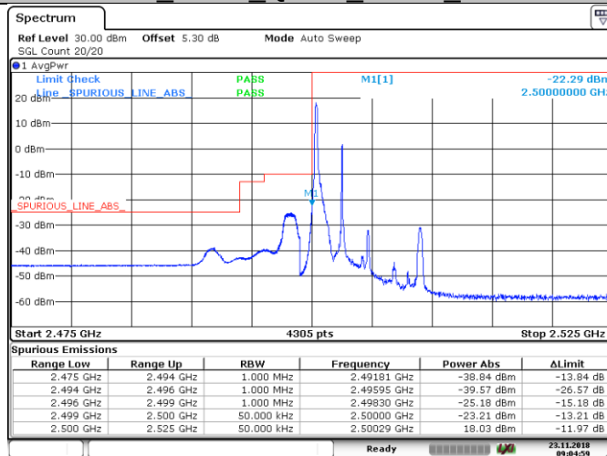
Band7_5MHz_QPSK_20775_1RB#0
