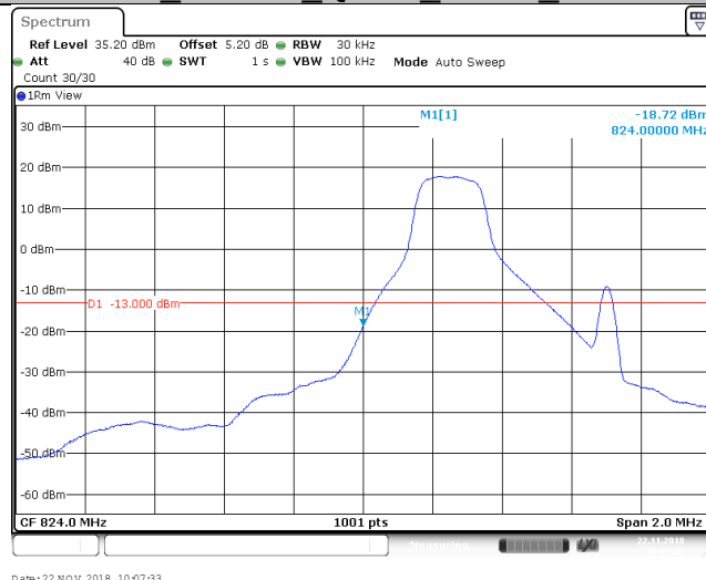
Band5 1.4MHz QPSK 20407 6RB#0
