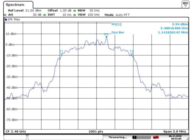
OBW_8DPSK_3DH5_2480MHz
