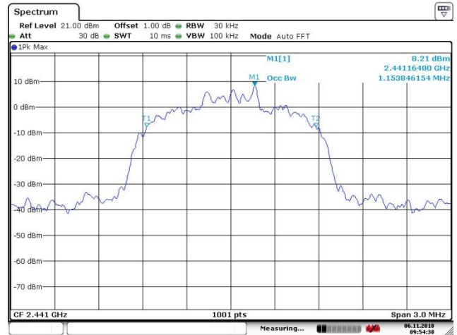
OBW_8DPSK_3DH5_2441MHz
