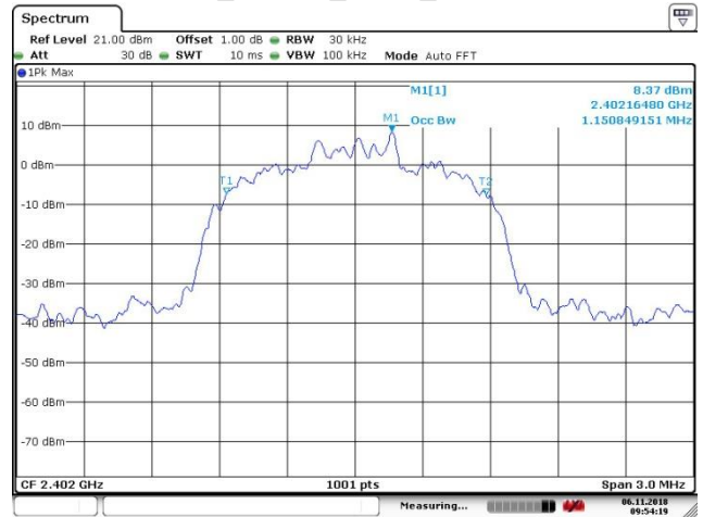
OBW_8DPSK_3DH5_2402MHz
