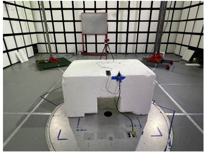
BL30 Setup 90 Degrees
