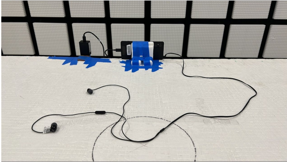
A1G Setup Front Mid Band
