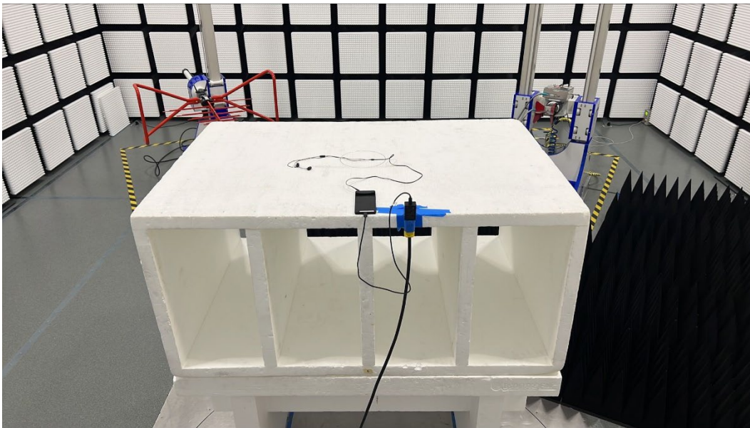
A1G Setup Back Low Band
