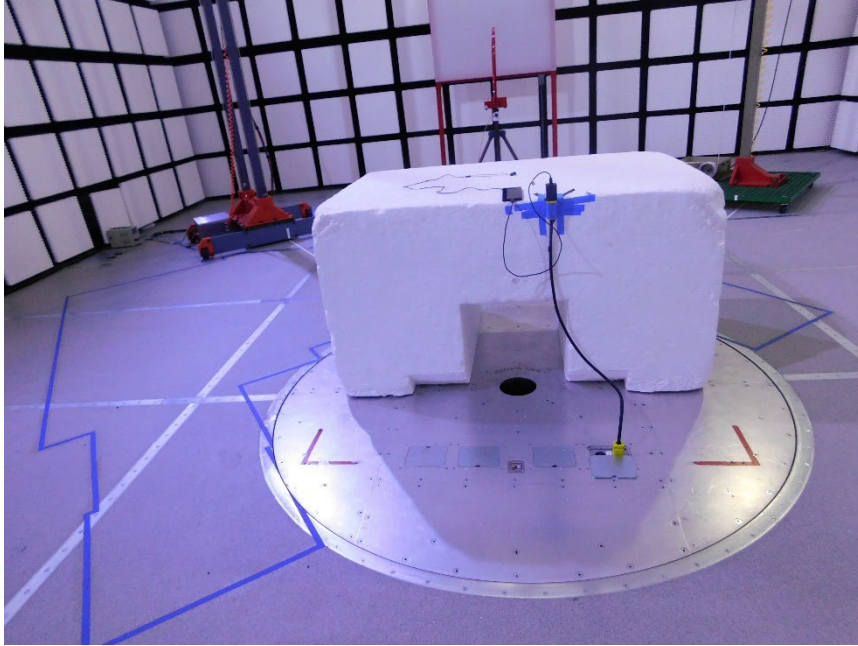
RADIATED PHOTO (<30 MHz 2.4 WLAN/BLE/BT CHAIN 0/1)
