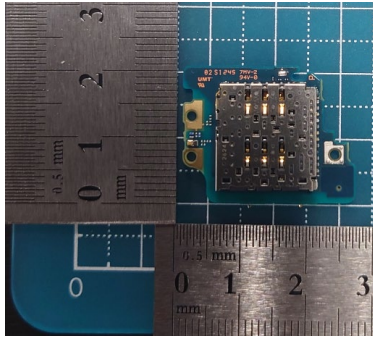
Internal Sub-PWB (Front-side)
