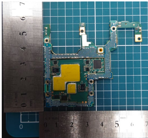
Only ② Rear PBA with Shield case (Front-side)
