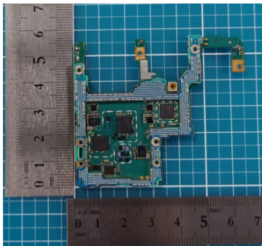
Only ② Rear PBA without Shield case (Front-side)
