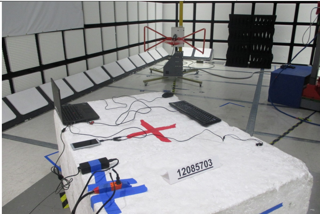
RADIATED BACK PHOTO (BELOW 1 GHz)
