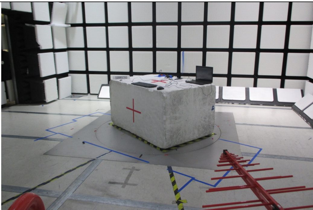
RADIATED FRONT PHOTO (BELOW 1 GHz)
